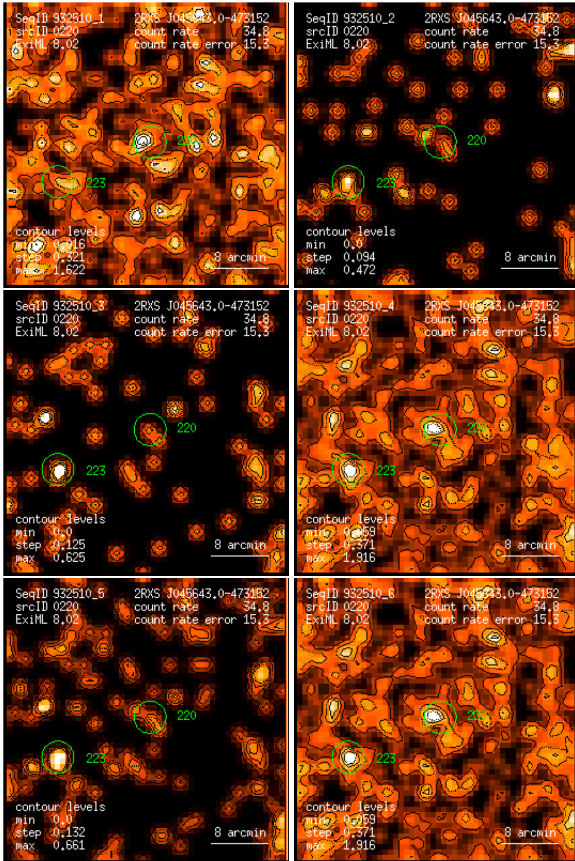
Figure 220: RASS 932510: detection 0220: band rate images, Gaussian filter: (1) PSPC channels 11 – 41, (2) 52 – 90, (3) 91 – 201, (4) 11 – 235, (5) 52 – 201, (6) 11 – 201. Broad band rates in counts/ks. Band rate contour levels in counts/ks/arcmin 2 .
