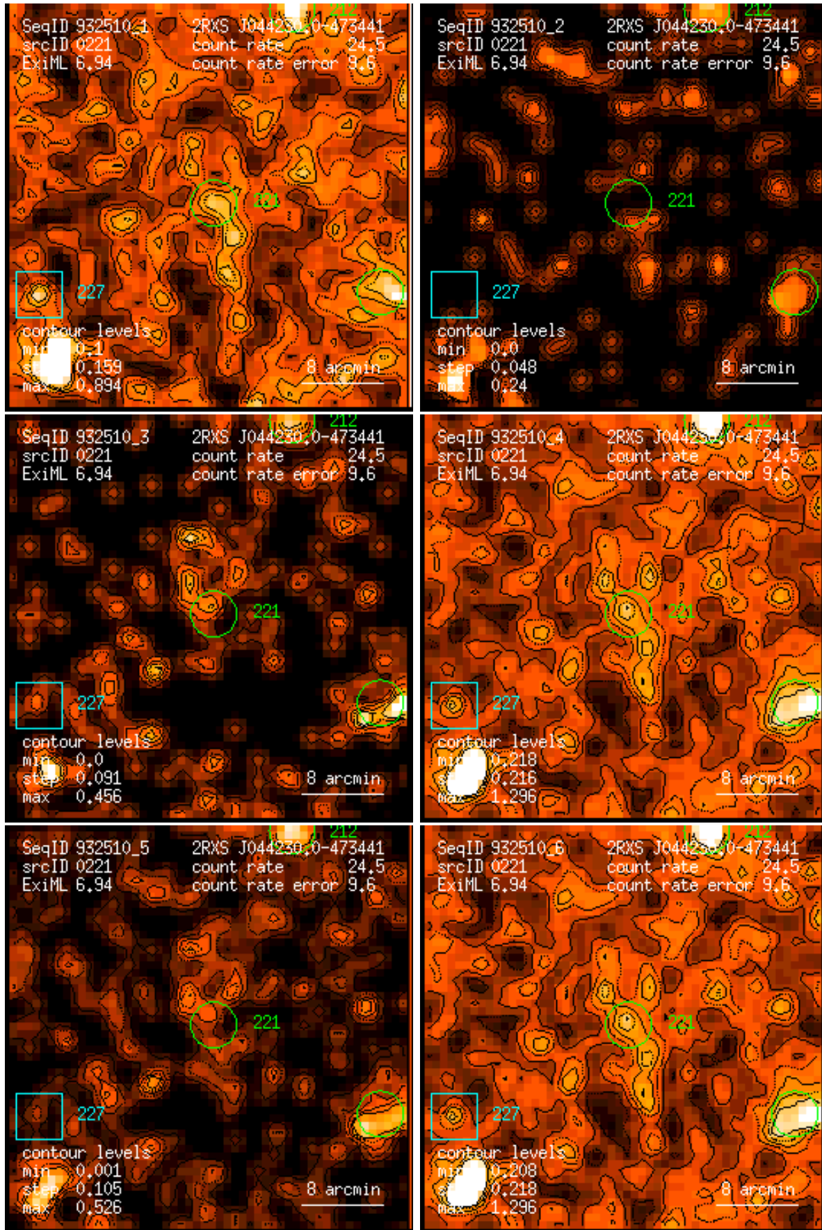
Figure 221: RASS 932510: detection 0221: band rate images, Gaussian filter: (1) PSPC channels 11 – 41, (2) 52 – 90, (3) 91 – 201, (4) 11 – 235, (5) 52 – 201, (6) 11 – 201. Broad band rates in counts/ks. Band rate contour levels in counts/ks/arcmin 2 .
