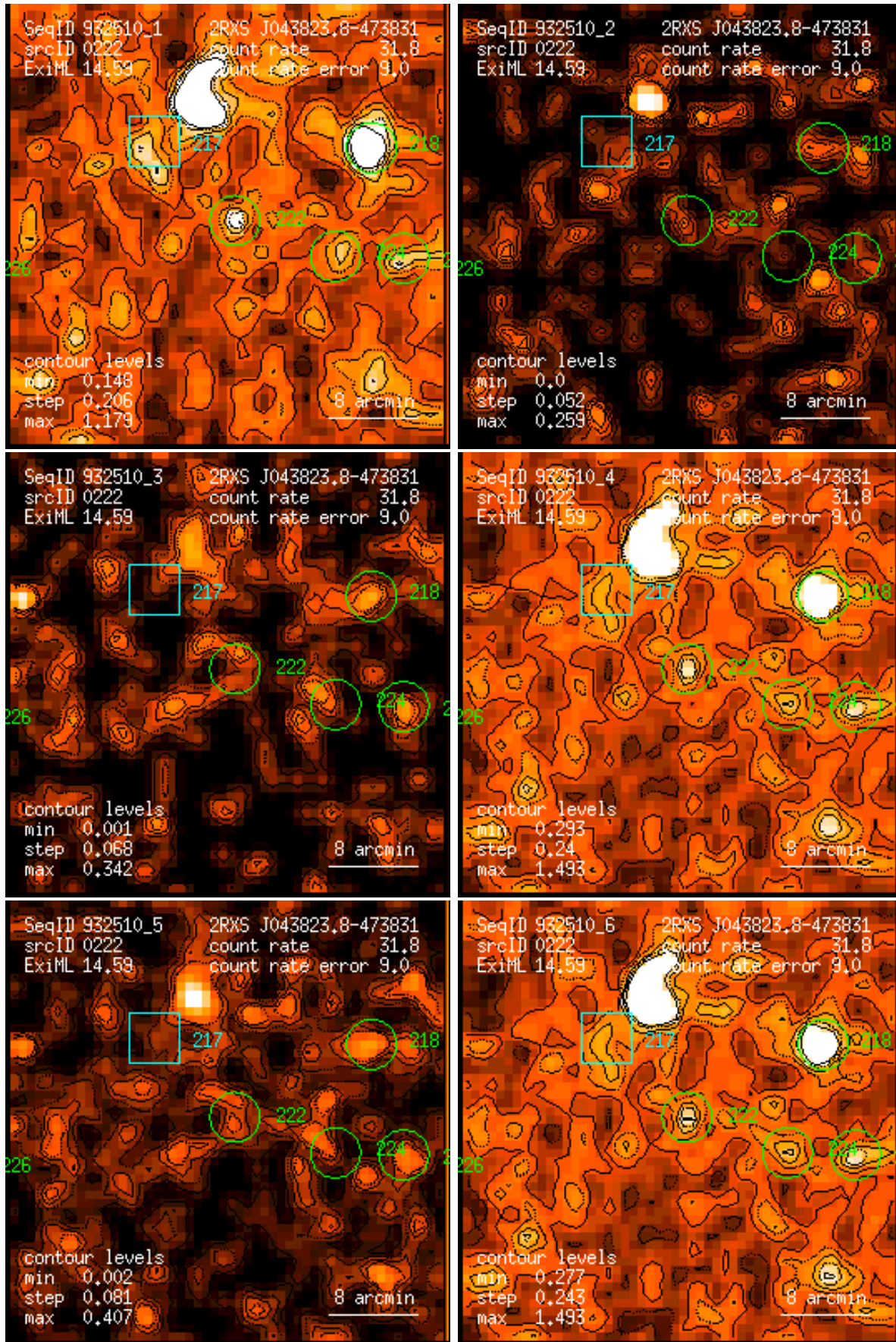
Figure 222: RASS 932510: detection 0222: band rate images, Gaussian filter: (1) PSPC channels 11 – 41, (2) 52 – 90, (3) 91 – 201, (4) 11 – 235, (5) 52 – 201, (6) 11 – 201. Broad band rates in counts/ks. Band rate contour levels in counts/ks/arcmin 2 .
