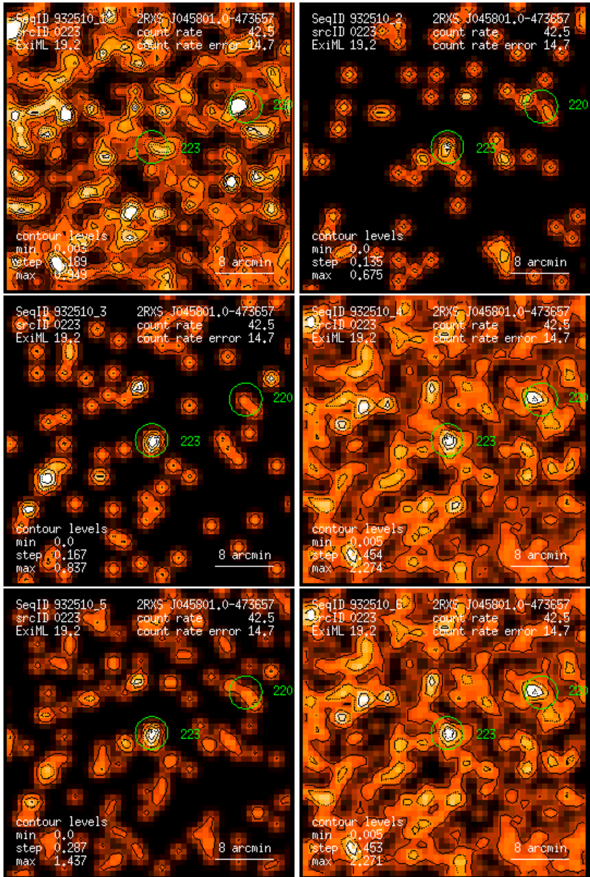
Figure 223: RASS 932510: detection 0223: band rate images, Gaussian filter: (1) PSPC channels 11 – 41, (2) 52 – 90, (3) 91 – 201, (4) 11 – 235, (5) 52 – 201, (6) 11 – 201. Broad band rates in counts/ks. Band rate contour levels in counts/ks/arcmin 2 .
