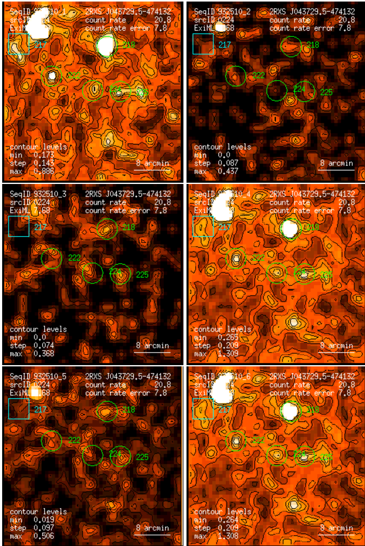
Figure 224: RASS 932510: detection 0224: band rate images, Gaussian filter: (1) PSPC channels 11 – 41, (2) 52 – 90, (3) 91 – 201, (4) 11 – 235, (5) 52 – 201, (6) 11 – 201. Broad band rates in counts/ks. Band rate contour levels in counts/ks/arcmin 2 .
