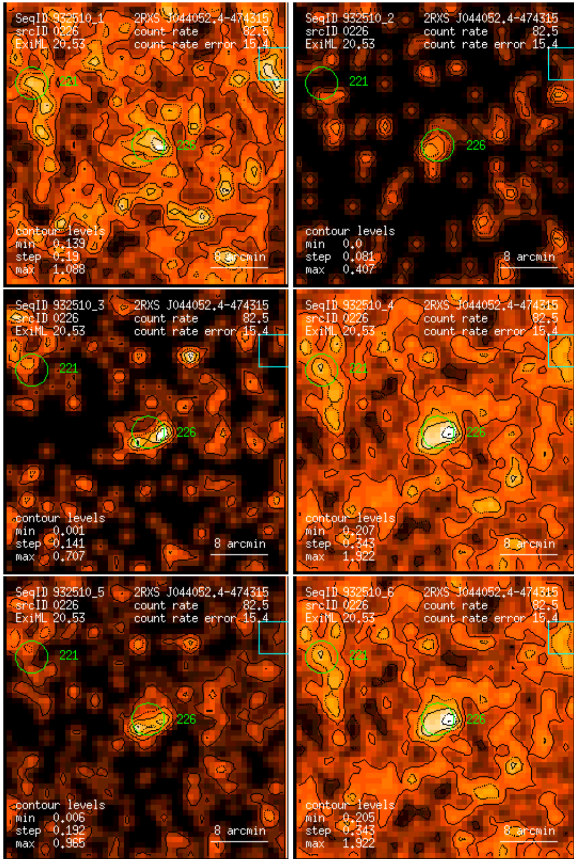
Figure 226: RASS 932510: detection 0226: band rate images, Gaussian filter: (1) PSPC channels 11 – 41, (2) 52 – 90, (3) 91 – 201, (4) 11 – 235, (5) 52 – 201, (6) 11 – 201. Broad band rates in counts/ks. Band rate contour levels in counts/ks/arcmin 2 .
