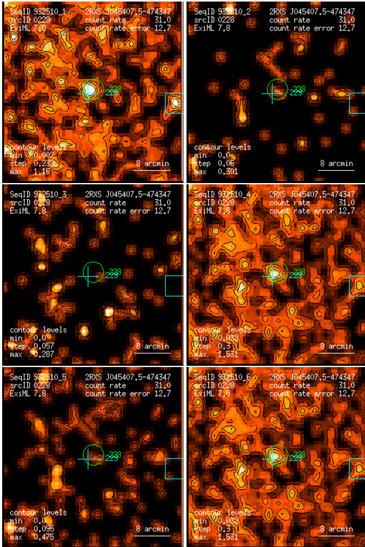
Figure 228: RASS 932510: detection 0228: band rate images, Gaussian filter: (1) PSPC channels 11 – 41, (2) 52 – 90, (3) 91 – 201, (4) 11 – 235, (5) 52 – 201, (6) 11 – 201. Broad band rates in counts/ks. Band rate contour levels in counts/ks/arcmin 2 .
