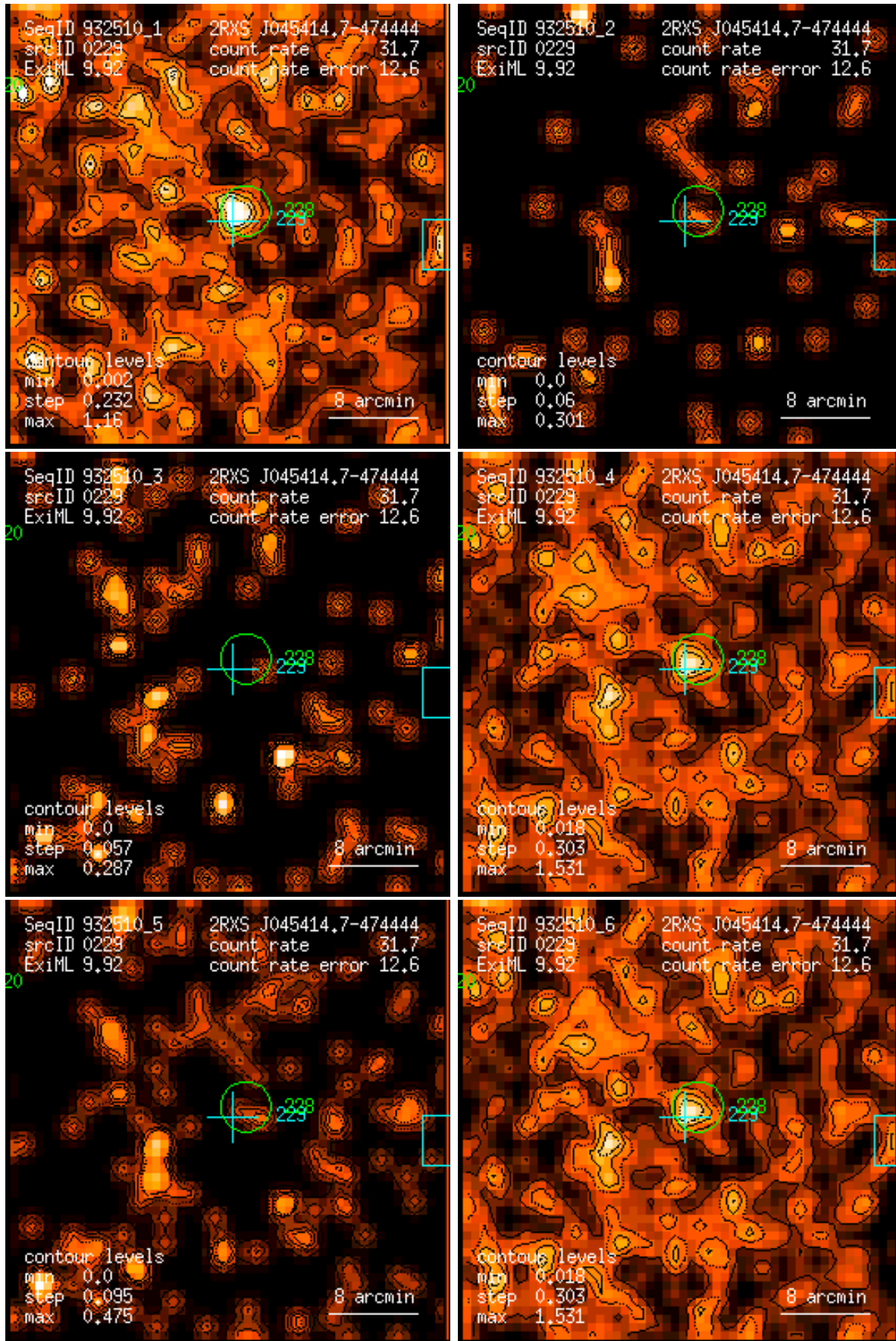
Figure 229: RASS 932510: detection 0229: band rate images, Gaussian filter: (1) PSPC channels 11 – 41, (2) 52 – 90, (3) 91 – 201, (4) 11 – 235, (5) 52 – 201, (6) 11 – 201. Broad band rates in counts/ks. Band rate contour levels in counts/ks/arcmin 2 .
