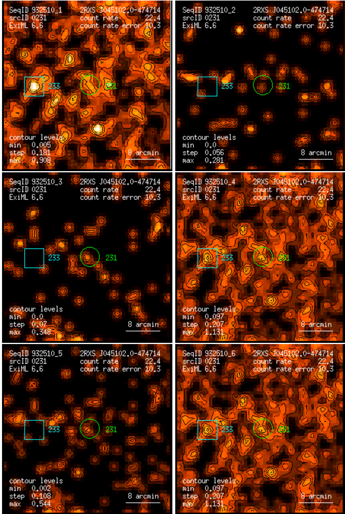
Figure 231: RASS 932510: detection 0231: band rate images, Gaussian filter: (1) PSPC channels 11 – 41, (2) 52 – 90, (3) 91 – 201, (4) 11 – 235, (5) 52 – 201, (6) 11 – 201. Broad band rates in counts/ks. Band rate contour levels in counts/ks/arcmin 2 .
