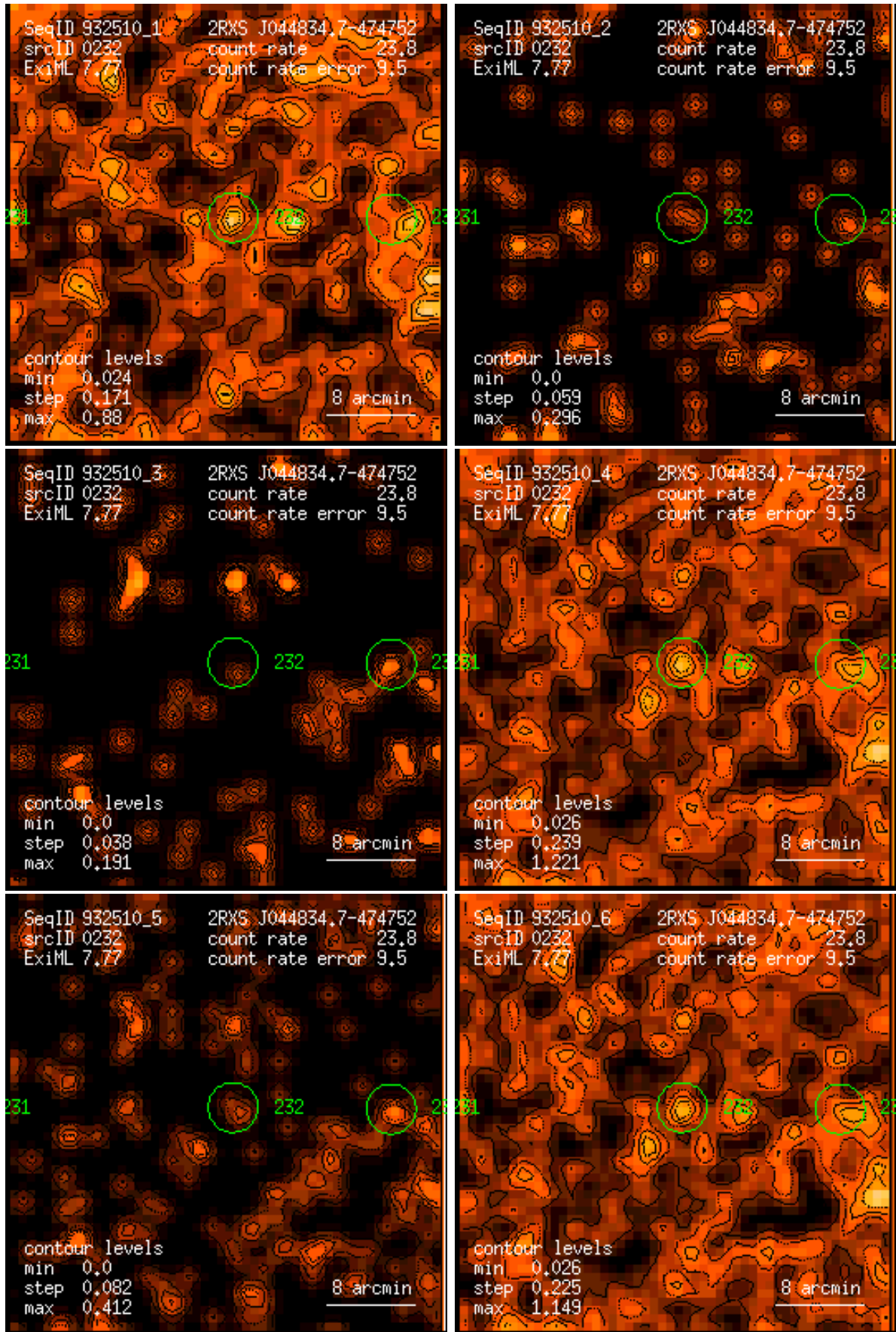
Figure 232: RASS 932510: detection 0232: band rate images, Gaussian filter: (1) PSPC channels 11 – 41, (2) 52 – 90, (3) 91 – 201, (4) 11 – 235, (5) 52 – 201, (6) 11 – 201. Broad band rates in counts/ks. Band rate contour levels in counts/ks/arcmin 2 .
