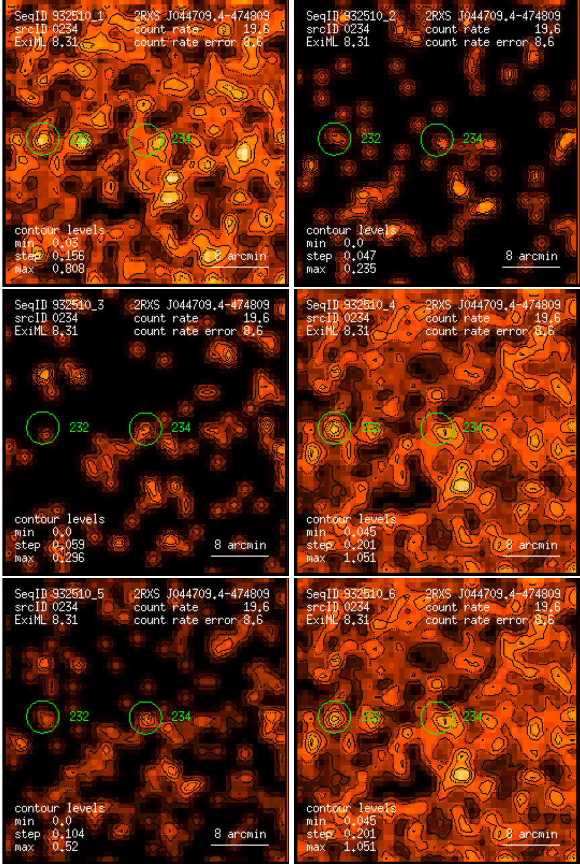
Figure 234: RASS 932510: detection 0234: band rate images, Gaussian filter: (1) PSPC channels 11 – 41, (2) 52 – 90, (3) 91 – 201, (4) 11 – 235, (5) 52 – 201, (6) 11 – 201. Broad band rates in counts/ks. Band rate contour levels in counts/ks/arcmin 2 .
