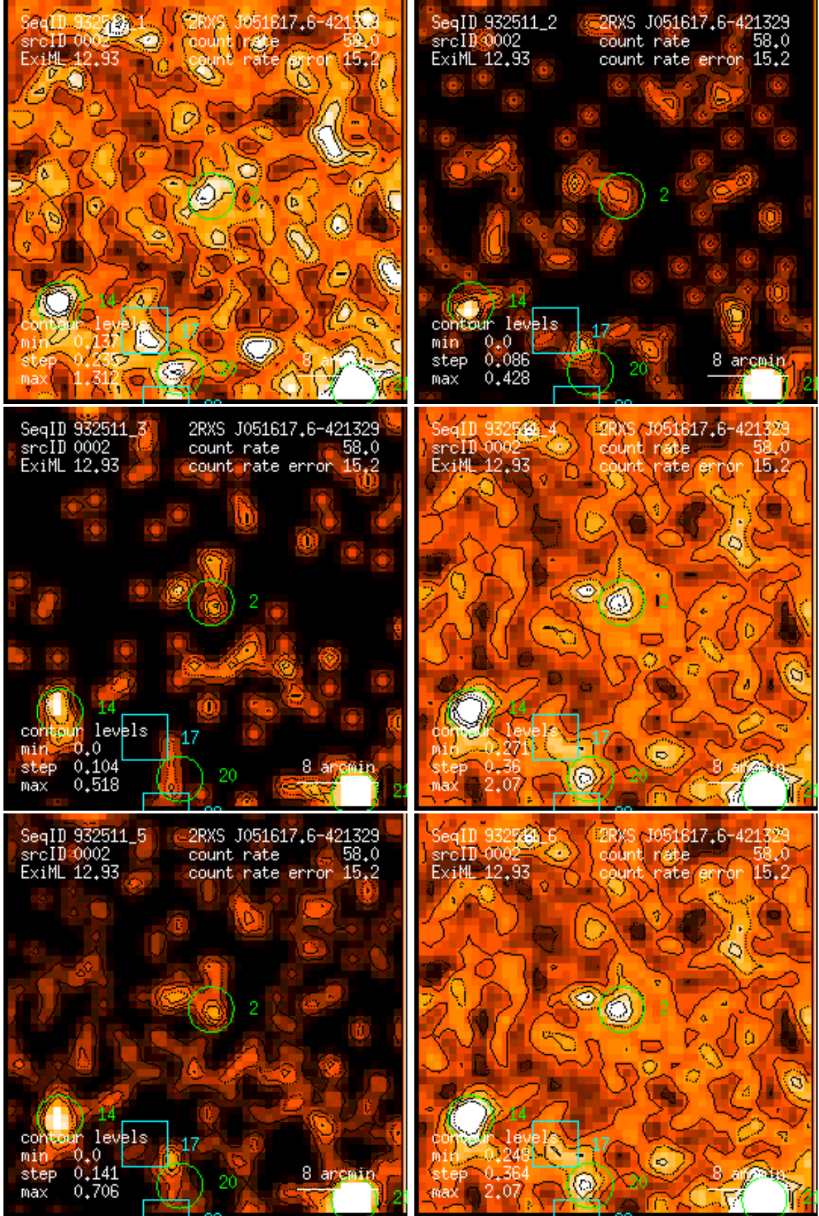
Figure 2: RASS 932511: detection 0002: band rate images, Gaussian filter: (1) PSPC channels 11 – 41, (2) 52 – 90, (3) 91 – 201, (4) 11 – 235, (5) 52 – 201, (6) 11 – 201. Broad band rates in counts/ks. Band rate contour levels in counts/ks/arcmin 2 .
