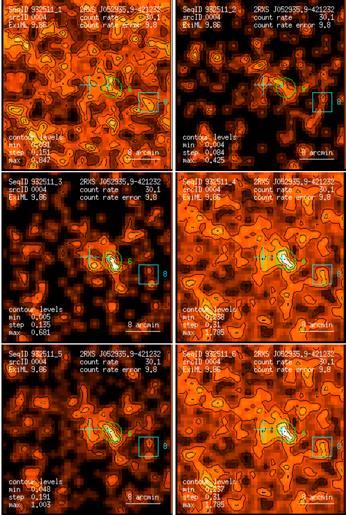
Figure 4: RASS 932511: detection 0004: band rate images, Gaussian filter: (1) PSPC channels 11 – 41, (2) 52 – 90, (3) 91 – 201, (4) 11 – 235, (5) 52 – 201, (6) 11 – 201. Broad band rates in counts/ks. Band rate contour levels in counts/ks/arcmin 2 .
