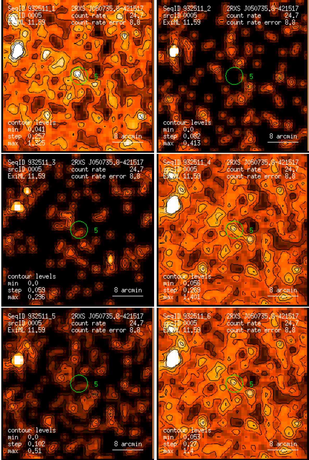
Figure 5: RASS 932511: detection 0005: band rate images, Gaussian filter: (1) PSPC channels 11 – 41, (2) 52 – 90, (3) 91 – 201, (4) 11 – 235, (5) 52 – 201, (6) 11 – 201. Broad band rates in counts/ks. Band rate contour levels in counts/ks/arcmin 2 .
