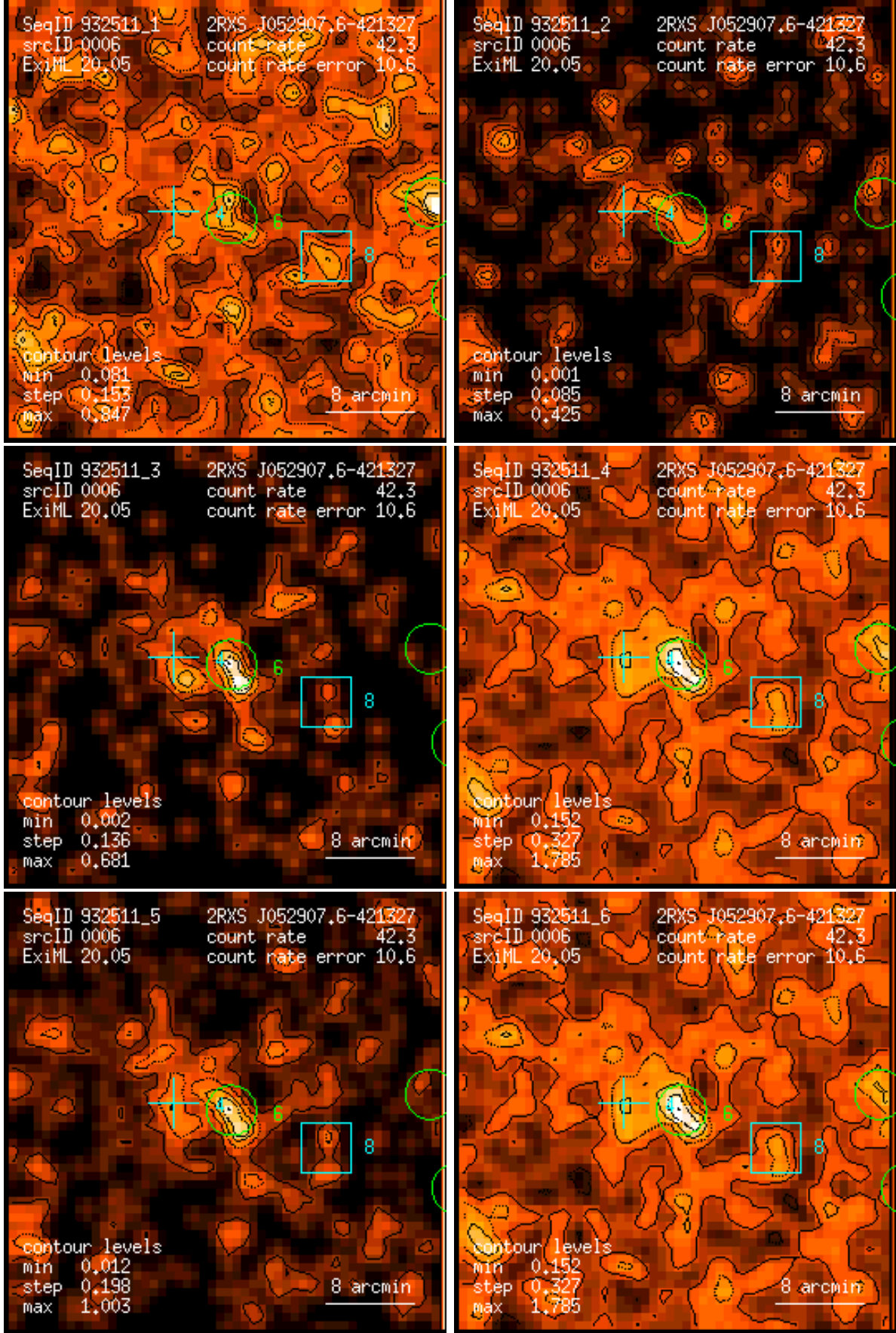
Figure 6: RASS 932511: detection 0006: band rate images, Gaussian filter: (1) PSPC channels 11 – 41, (2) 52 – 90, (3) 91 – 201, (4) 11 – 235, (5) 52 – 201, (6) 11 – 201. Broad band rates in counts/ks. Band rate contour levels in counts/ks/arcmin 2 .
