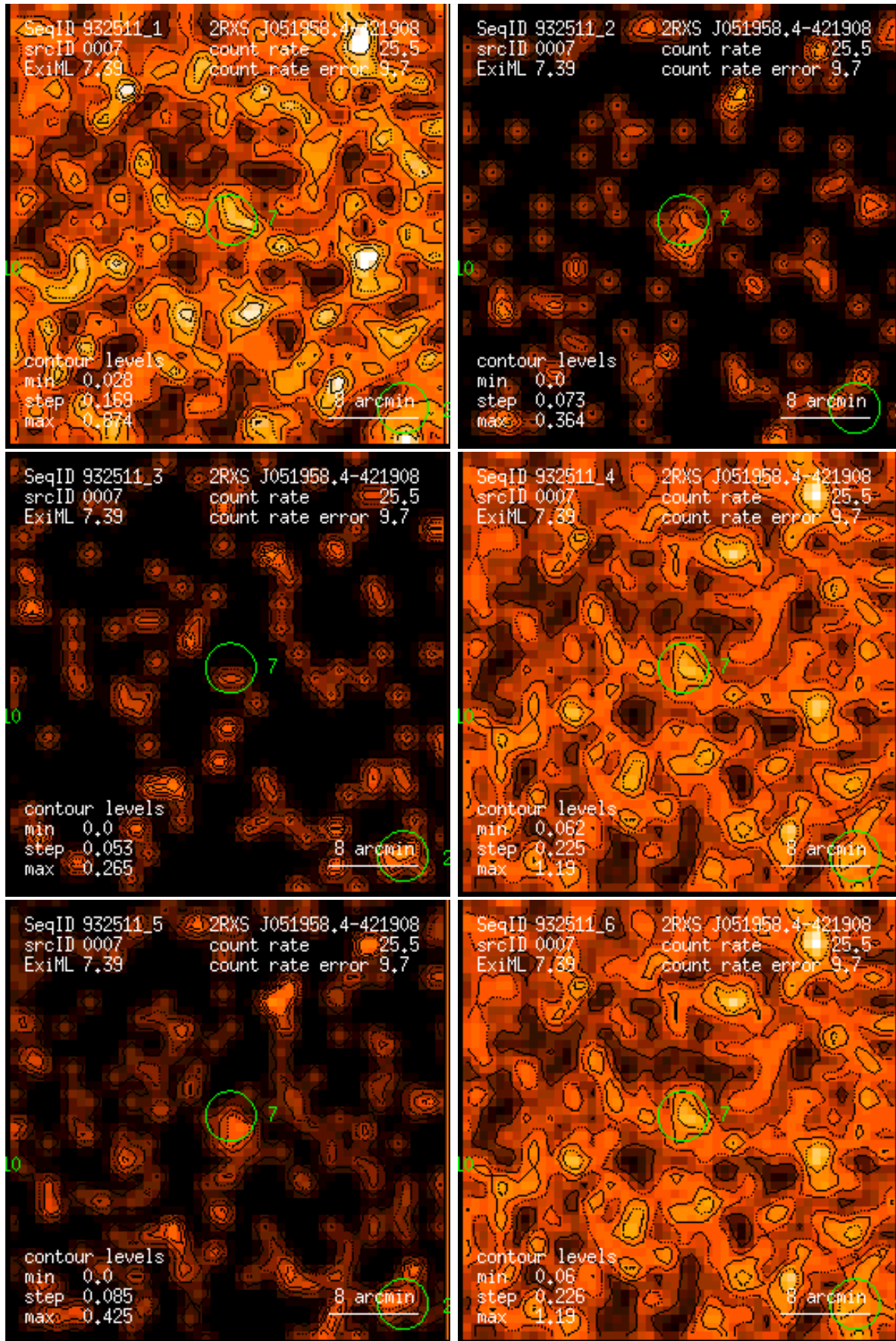
Figure 7: RASS 932511: detection 0007: band rate images, Gaussian filter: (1) PSPC channels 11 – 41, (2) 52 – 90, (3) 91 – 201, (4) 11 – 235, (5) 52 – 201, (6) 11 – 201. Broad band rates in counts/ks. Band rate contour levels in counts/ks/arcmin 2 .
