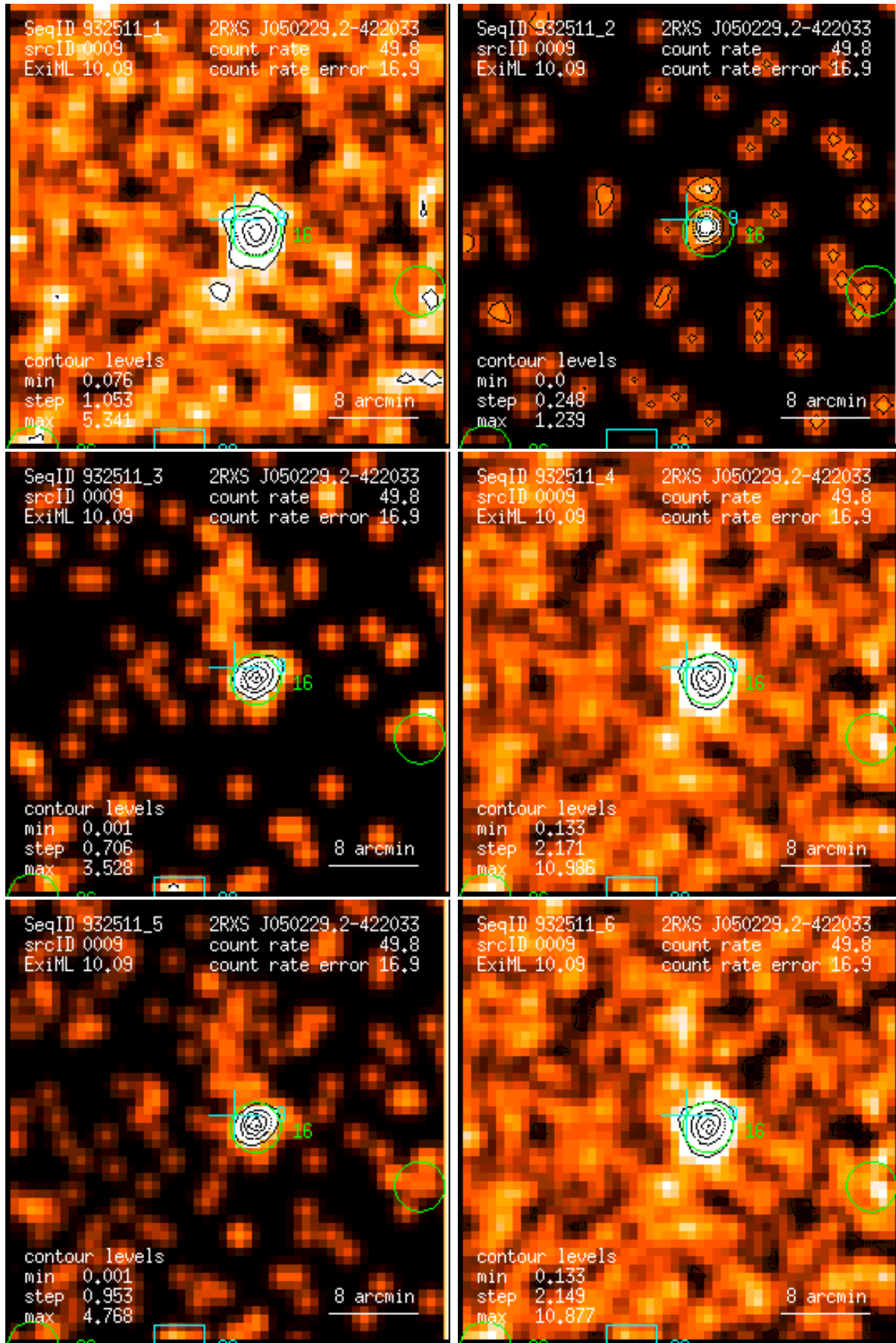
Figure 9: RASS 932511: detection 0009: band rate images, Gaussian filter: (1) PSPC channels 11 – 41, (2) 52 – 90, (3) 91 – 201, (4) 11 – 235, (5) 52 – 201, (6) 11 – 201. Broad band rates in counts/ks. Band rate contour levels in counts/ks/arcmin 2 .
