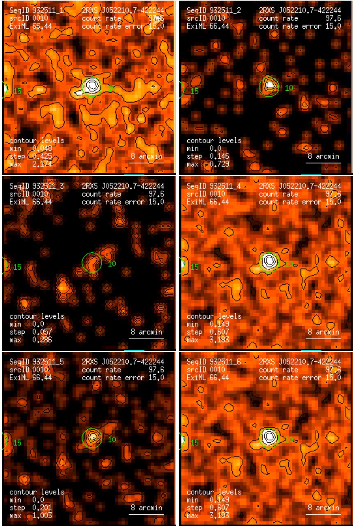
Figure 10: RASS 932511: detection 0010: band rate images, Gaussian filter: (1) PSPC channels 11 – 41, (2) 52 – 90, (3) 91 – 201, (4) 11 – 235, (5) 52 – 201, (6) 11 – 201. Broad band rates in counts/ks. Band rate contour levels in counts/ks/arcmin 2 .
