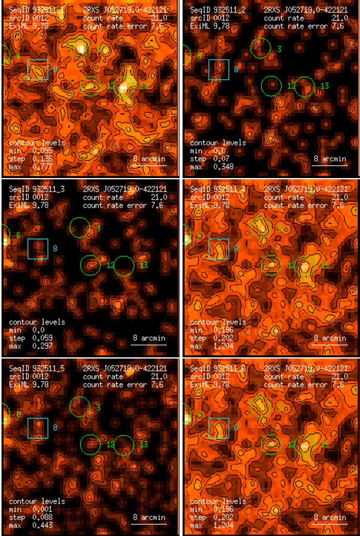
Figure 12: RASS 932511: detection 0012: band rate images, Gaussian filter: (1) PSPC channels 11 – 41, (2) 52 – 90, (3) 91 – 201, (4) 11 – 235, (5) 52 – 201, (6) 11 – 201. Broad band rates in counts/ks. Band rate contour levels in counts/ks/arcmin 2 .
