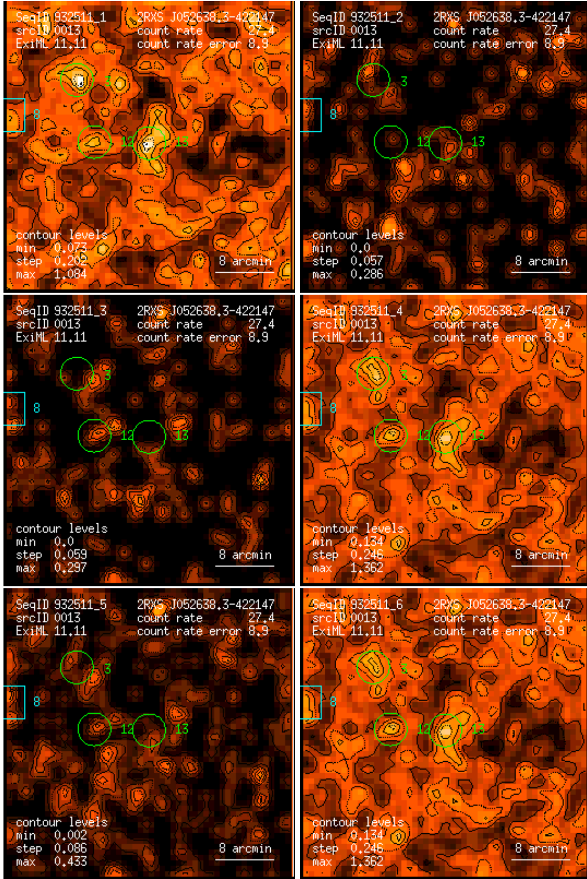
Figure 13: RASS 932511: detection 0013: band rate images, Gaussian filter: (1) PSPC channels 11 – 41, (2) 52 – 90, (3) 91 – 201, (4) 11 – 235, (5) 52 – 201, (6) 11 – 201. Broad band rates in counts/ks. Band rate contour levels in counts/ks/arcmin 2 .
