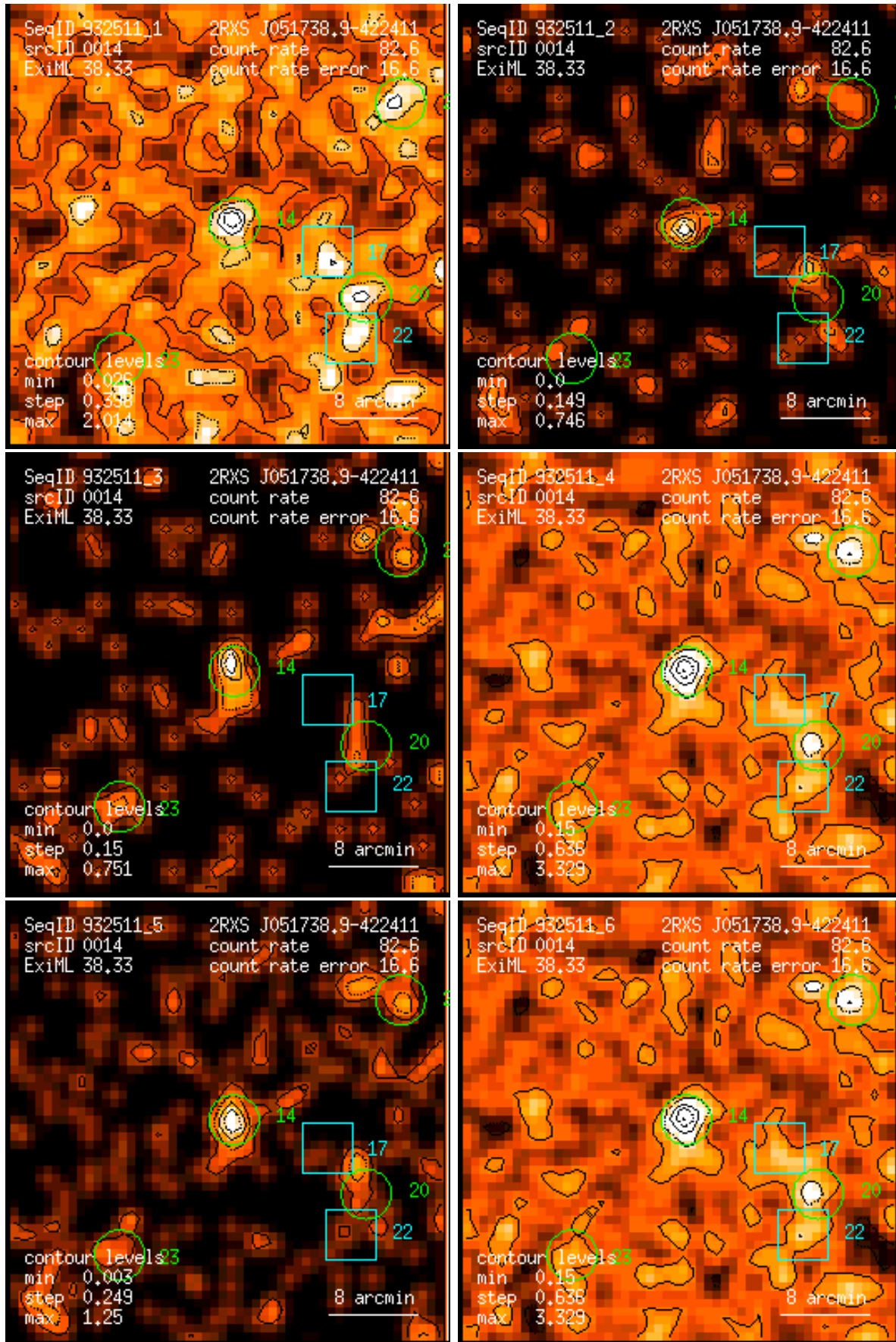
Figure 14: RASS 932511: detection 0014: band rate images, Gaussian filter: (1) PSPC channels 11 – 41, (2) 52 – 90, (3) 91 – 201, (4) 11 – 235, (5) 52 – 201, (6) 11 – 201. Broad band rates in counts/ks. Band rate contour levels in counts/ks/arcmin 2 .
