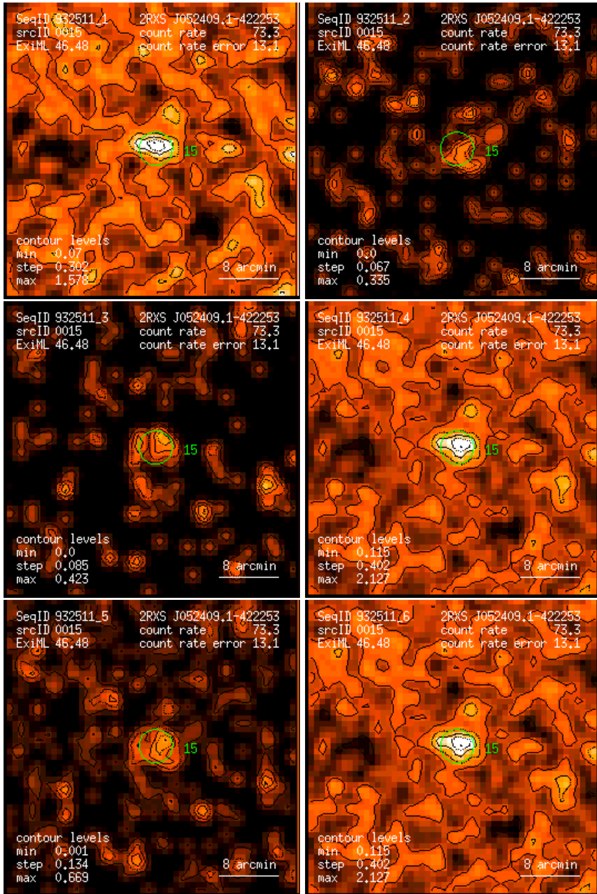
Figure 15: RASS 932511: detection 0015: band rate images, Gaussian filter: (1) PSPC channels 11 – 41, (2) 52 – 90, (3) 91 – 201, (4) 11 – 235, (5) 52 – 201, (6) 11 – 201. Broad band rates in counts/ks. Band rate contour levels in counts/ks/arcmin 2 .
