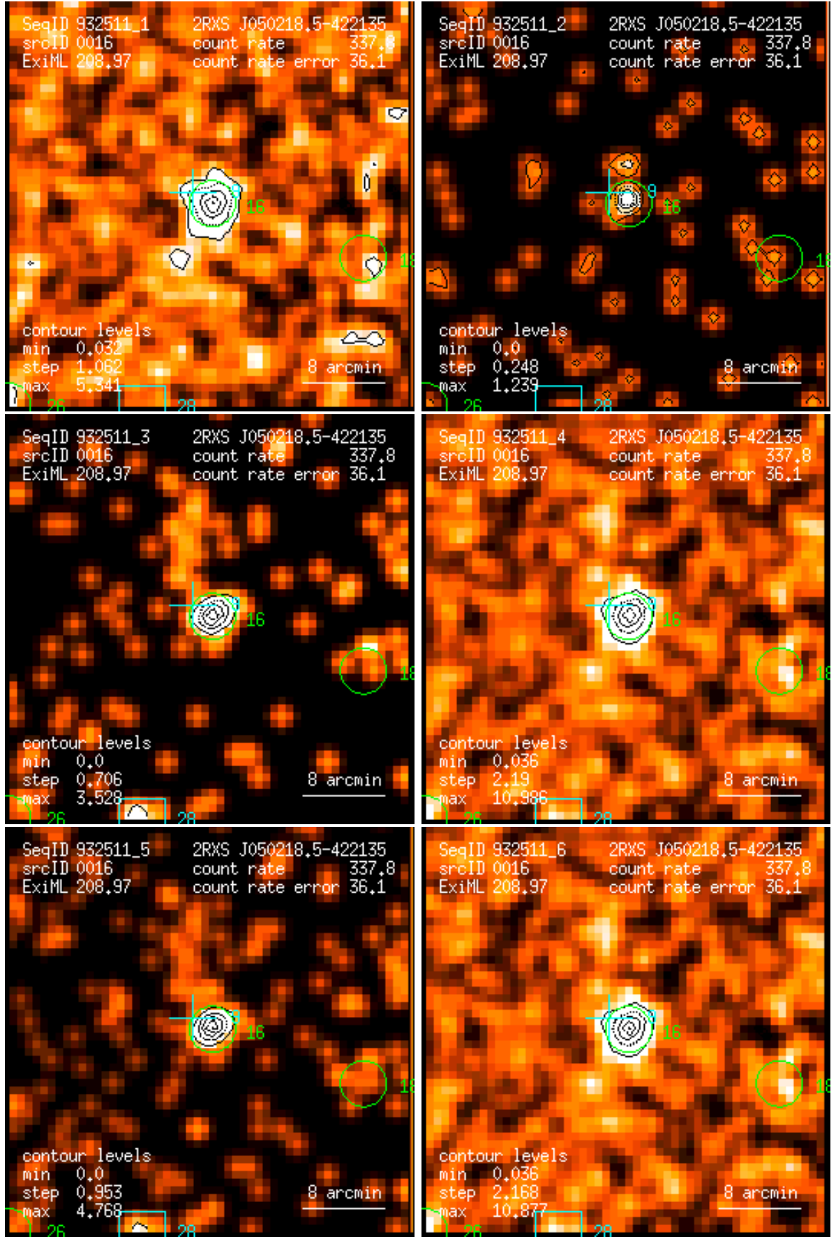
Figure 16: RASS 932511: detection 0016: band rate images, Gaussian filter: (1) PSPC channels 11 – 41, (2) 52 – 90, (3) 91 – 201, (4) 11 – 235, (5) 52 – 201, (6) 11 – 201. Broad band rates in counts/ks. Band rate contour levels in counts/ks/arcmin 2 .
