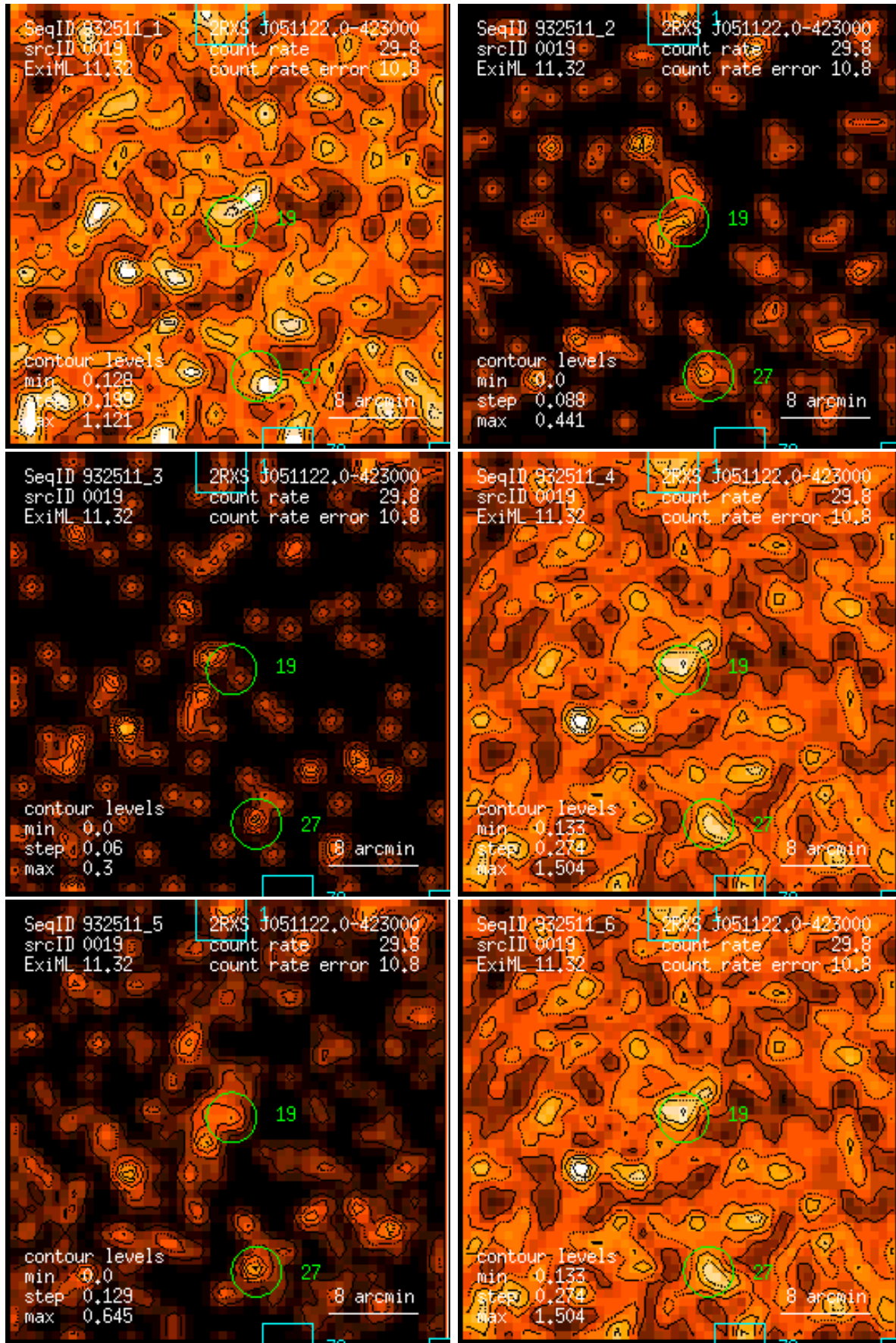
Figure 19: RASS 932511: detection 0019: band rate images, Gaussian filter: (1) PSPC channels 11 – 41, (2) 52 – 90, (3) 91 – 201, (4) 11 – 235, (5) 52 – 201, (6) 11 – 201. Broad band rates in counts/ks. Band rate contour levels in counts/ks/arcmin 2 .
