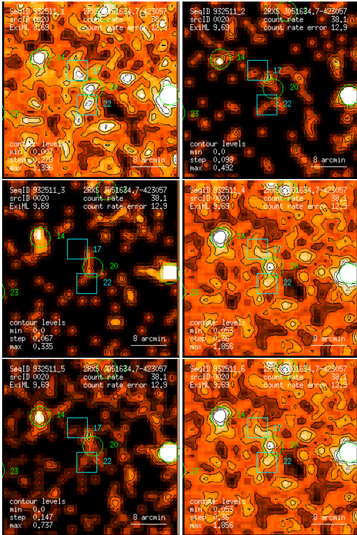
Figure 20: RASS 932511: detection 0020: band rate images, Gaussian filter: (1) PSPC channels 11 – 41, (2) 52 – 90, (3) 91 – 201, (4) 11 – 235, (5) 52 – 201, (6) 11 – 201. Broad band rates in counts/ks. Band rate contour levels in counts/ks/arcmin 2 .
