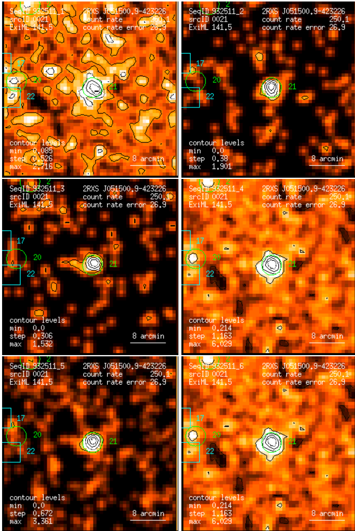
Figure 21: RASS 932511: detection 0021: band rate images, Gaussian filter: (1) PSPC channels 11 – 41, (2) 52 – 90, (3) 91 – 201, (4) 11 – 235, (5) 52 – 201, (6) 11 – 201. Broad band rates in counts/ks. Band rate contour levels in counts/ks/arcmin 2 .
