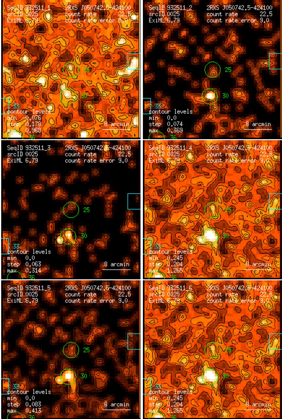
Figure 25: RASS 932511: detection 0025: band rate images, Gaussian filter: (1) PSPC channels 11 – 41, (2) 52 – 90, (3) 91 – 201, (4) 11 – 235, (5) 52 – 201, (6) 11 – 201. Broad band rates in counts/ks. Band rate contour levels in counts/ks/arcmin 2 .
