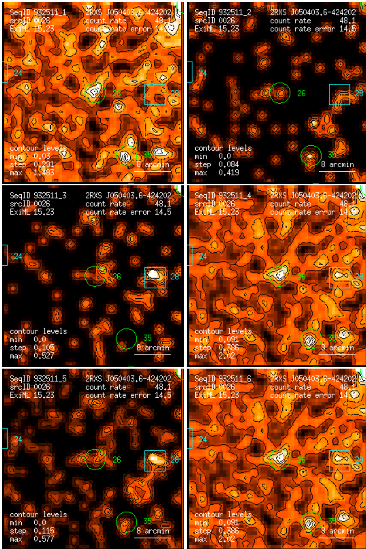
Figure 26: RASS 932511: detection 0026: band rate images, Gaussian filter: (1) PSPC channels 11 – 41, (2) 52 – 90, (3) 91 – 201, (4) 11 – 235, (5) 52 – 201, (6) 11 – 201. Broad band rates in counts/ks. Band rate contour levels in counts/ks/arcmin 2 .
