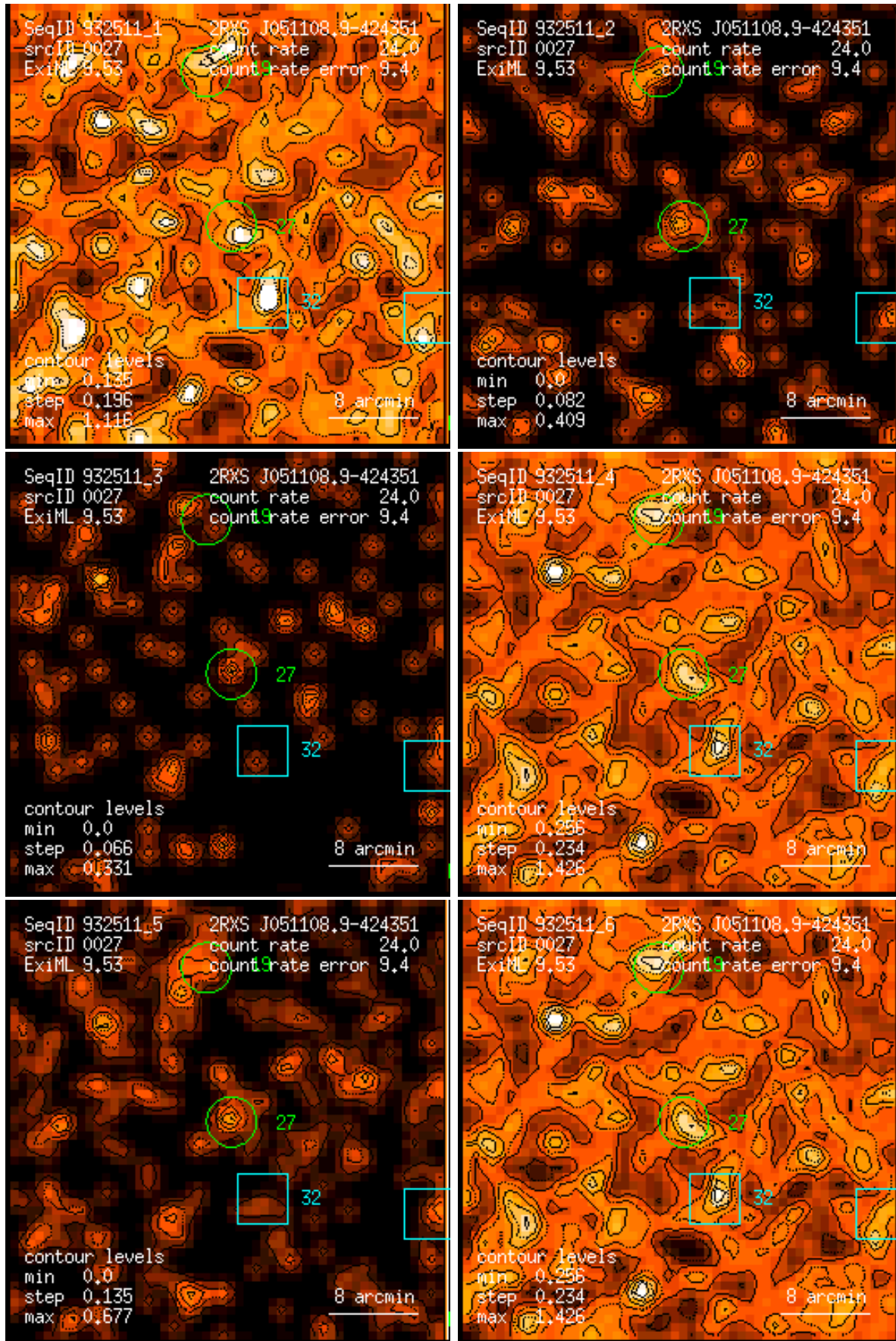
Figure 27: RASS 932511: detection 0027: band rate images, Gaussian filter: (1) PSPC channels 11 – 41, (2) 52 – 90, (3) 91 – 201, (4) 11 – 235, (5) 52 – 201, (6) 11 – 201. Broad band rates in counts/ks. Band rate contour levels in counts/ks/arcmin 2 .
