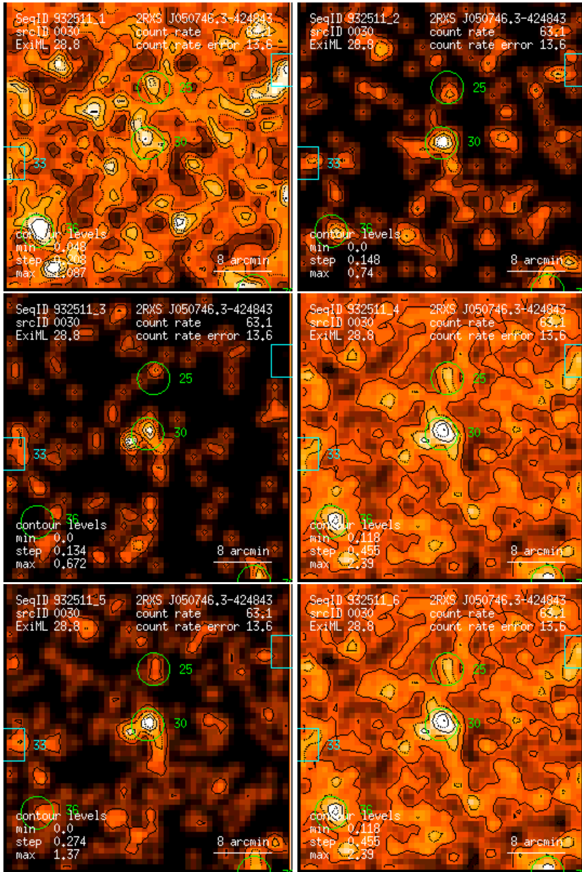
Figure 30: RASS 932511: detection 0030: band rate images, Gaussian filter: (1) PSPC channels 11 – 41, (2) 52 – 90, (3) 91 – 201, (4) 11 – 235, (5) 52 – 201, (6) 11 – 201. Broad band rates in counts/ks. Band rate contour levels in counts/ks/arcmin 2 .
