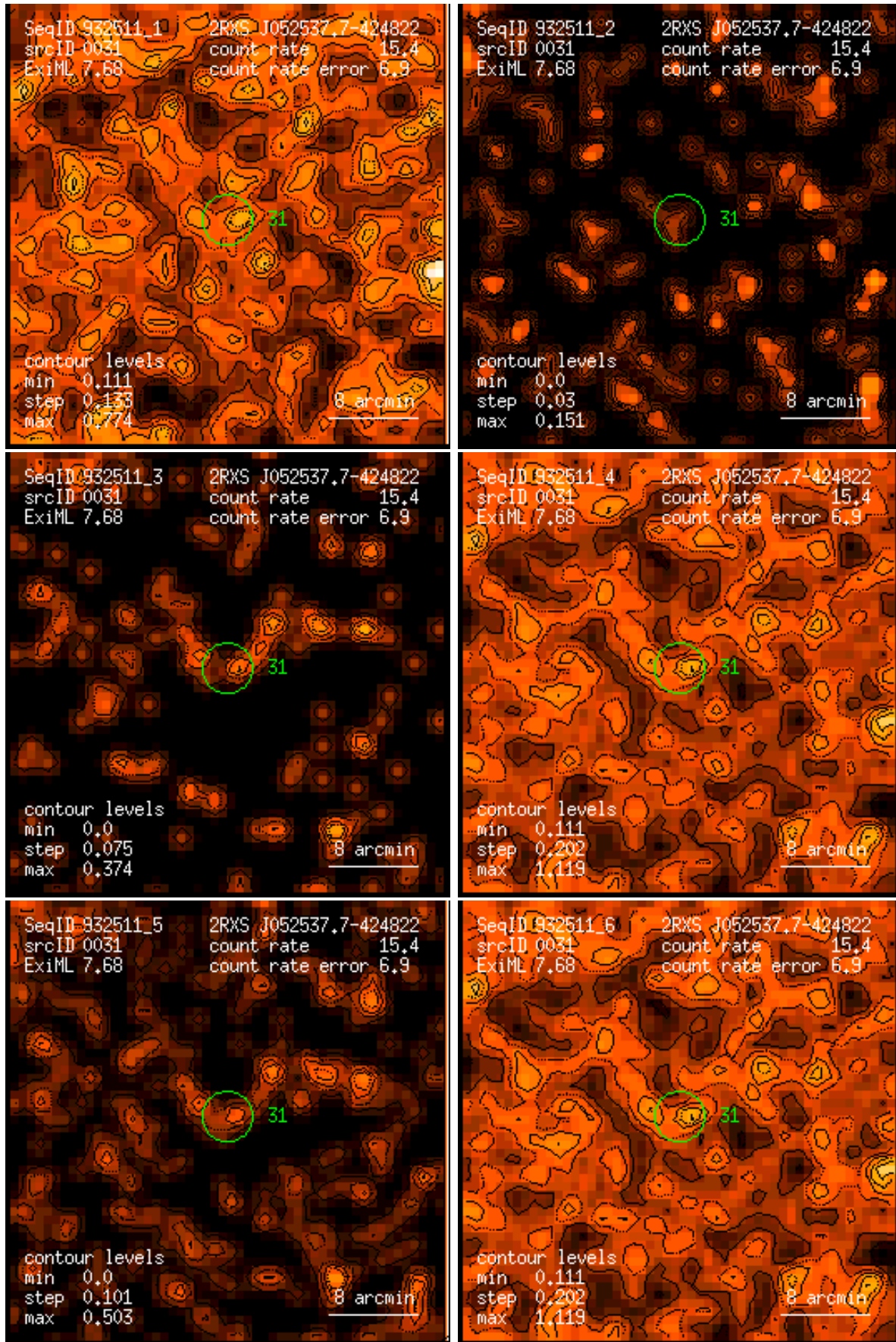
Figure 31: RASS 932511: detection 0031: band rate images, Gaussian filter: (1) PSPC channels 11 – 41, (2) 52 – 90, (3) 91 – 201, (4) 11 – 235, (5) 52 – 201, (6) 11 – 201. Broad band rates in counts/ks. Band rate contour levels in counts/ks/arcmin 2 .
