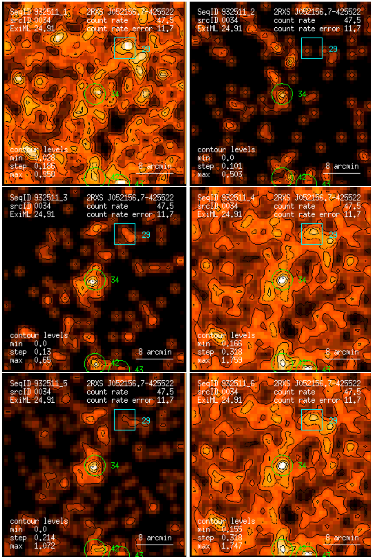
Figure 34: RASS 932511: detection 0034: band rate images, Gaussian filter: (1) PSPC channels 11 – 41, (2) 52 – 90, (3) 91 – 201, (4) 11 – 235, (5) 52 – 201, (6) 11 – 201. Broad band rates in counts/ks. Band rate contour levels in counts/ks/arcmin 2 .
