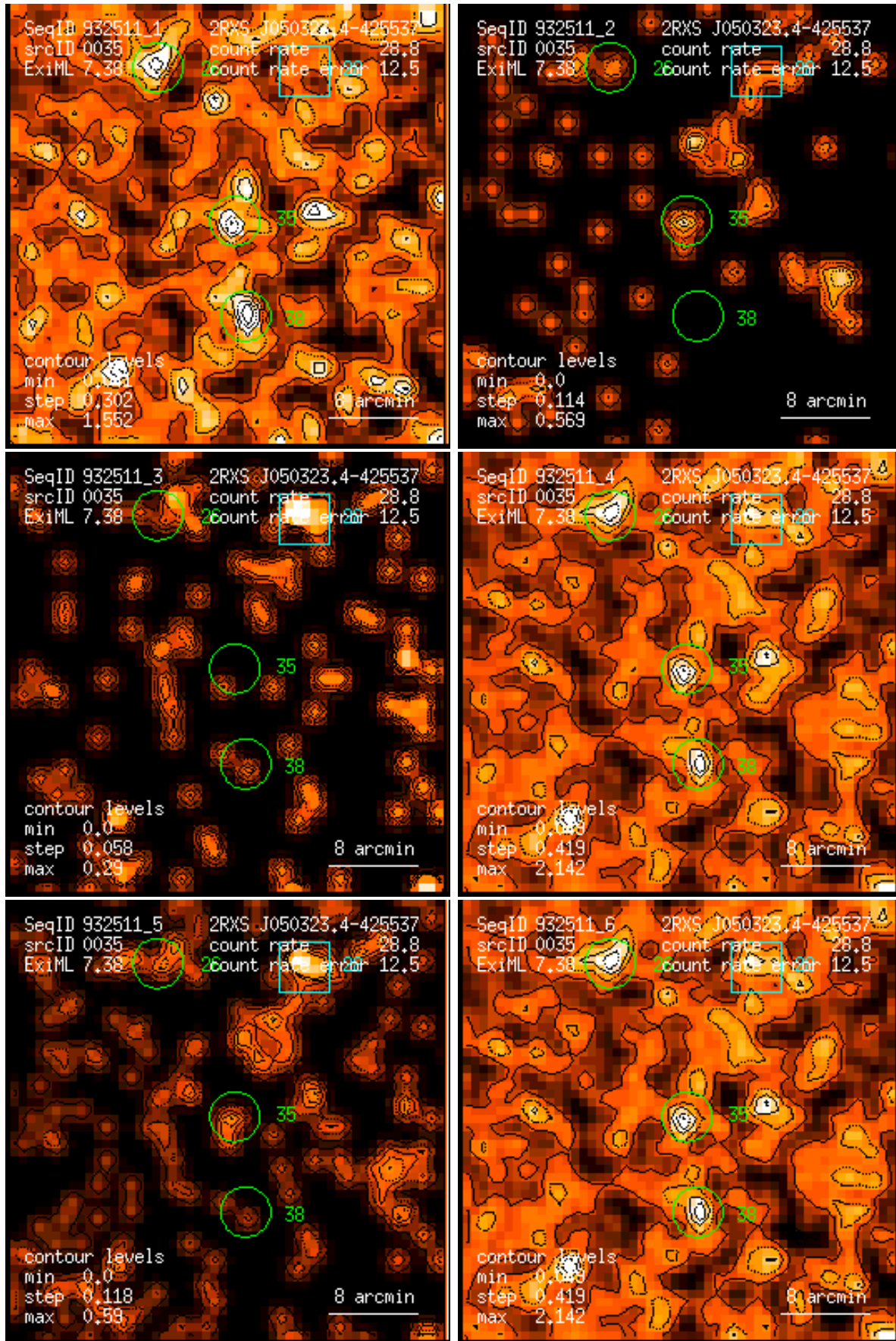
Figure 35: RASS 932511: detection 0035: band rate images, Gaussian filter: (1) PSPC channels 11 – 41, (2) 52 – 90, (3) 91 – 201, (4) 11 – 235, (5) 52 – 201, (6) 11 – 201. Broad band rates in counts/ks. Band rate contour levels in counts/ks/arcmin 2 .
