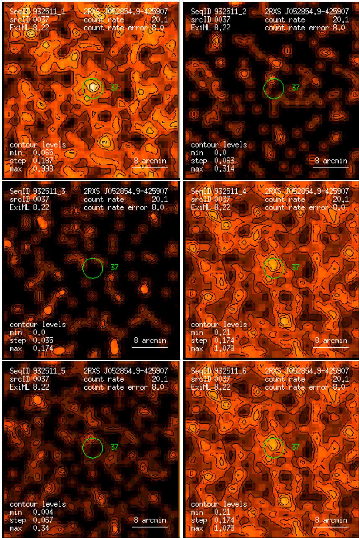
Figure 37: RASS 932511: detection 0037: band rate images, Gaussian filter: (1) PSPC channels 11 – 41, (2) 52 – 90, (3) 91 – 201, (4) 11 – 235, (5) 52 – 201, (6) 11 – 201. Broad band rates in counts/ks. Band rate contour levels in counts/ks/arcmin 2 .
