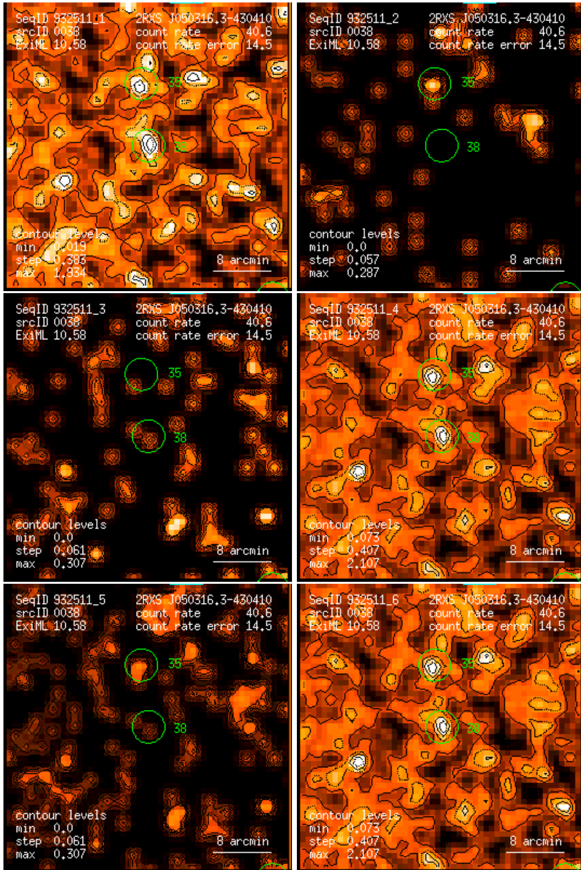
Figure 38: RASS 932511: detection 0038: band rate images, Gaussian filter: (1) PSPC channels 11 – 41, (2) 52 – 90, (3) 91 – 201, (4) 11 – 235, (5) 52 – 201, (6) 11 – 201. Broad band rates in counts/ks. Band rate contour levels in counts/ks/arcmin 2 .
