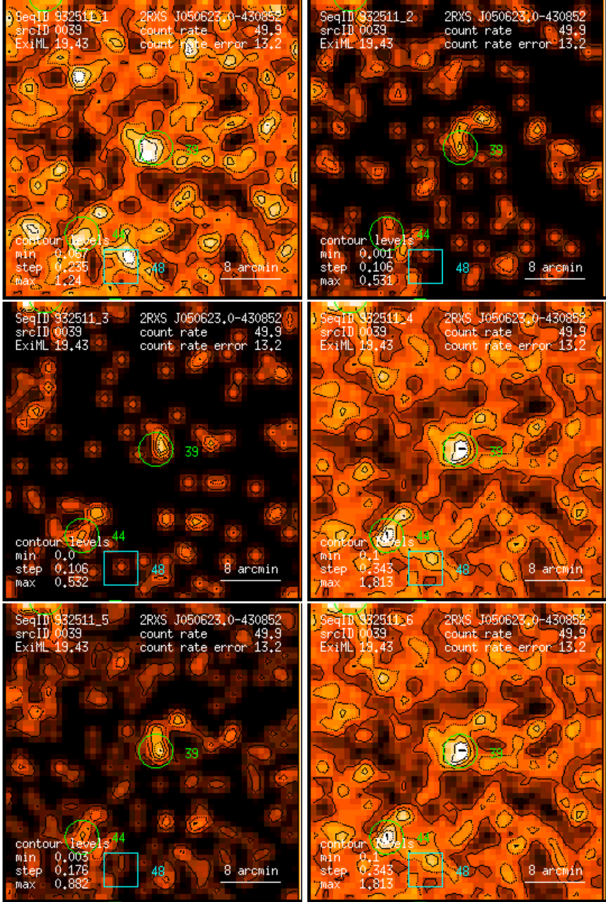
Figure 39: RASS 932511: detection 0039: band rate images, Gaussian filter: (1) PSPC channels 11 – 41, (2) 52 – 90, (3) 91 – 201, (4) 11 – 235, (5) 52 – 201, (6) 11 – 201. Broad band rates in counts/ks. Band rate contour levels in counts/ks/arcmin 2 .
