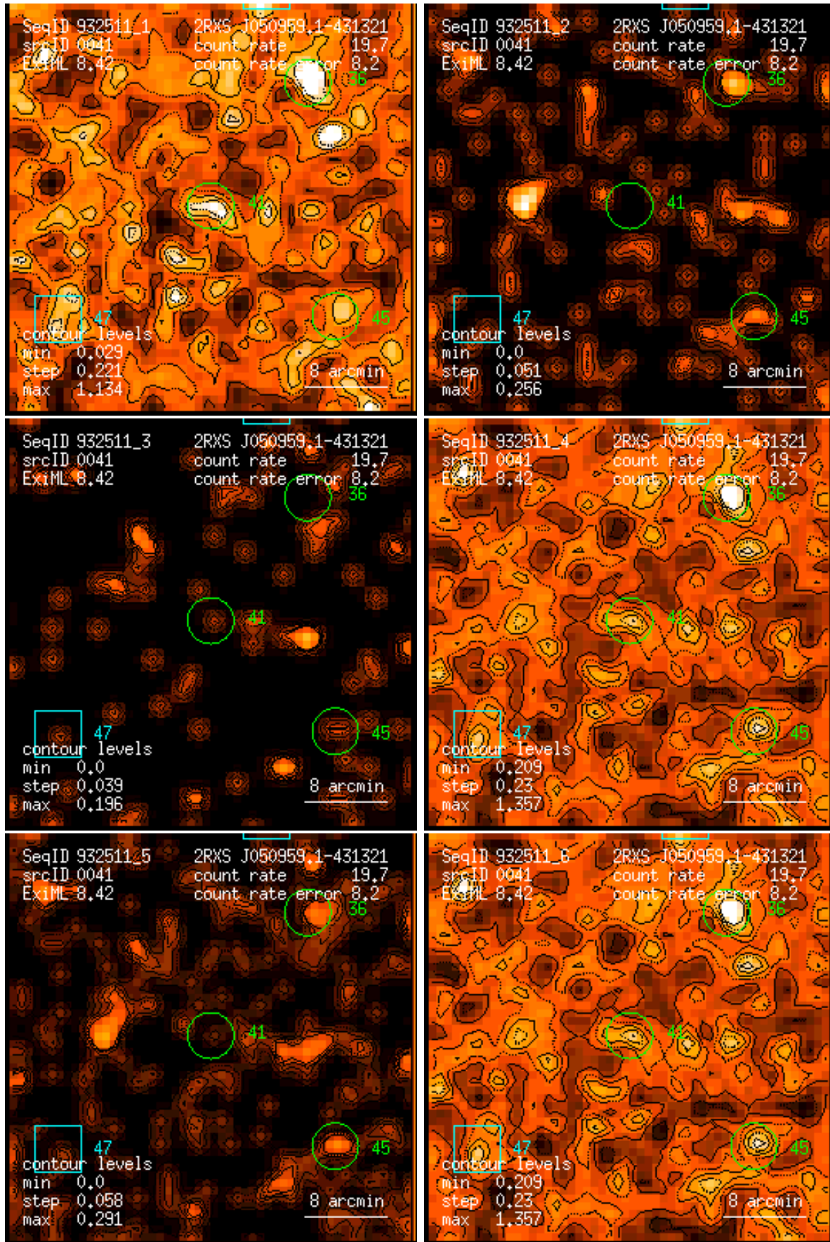
Figure 41: RASS 932511: detection 0041: band rate images, Gaussian filter: (1) PSPC channels 11 – 41, (2) 52 – 90, (3) 91 – 201, (4) 11 – 235, (5) 52 – 201, (6) 11 – 201. Broad band rates in counts/ks. Band rate contour levels in counts/ks/arcmin 2 .
