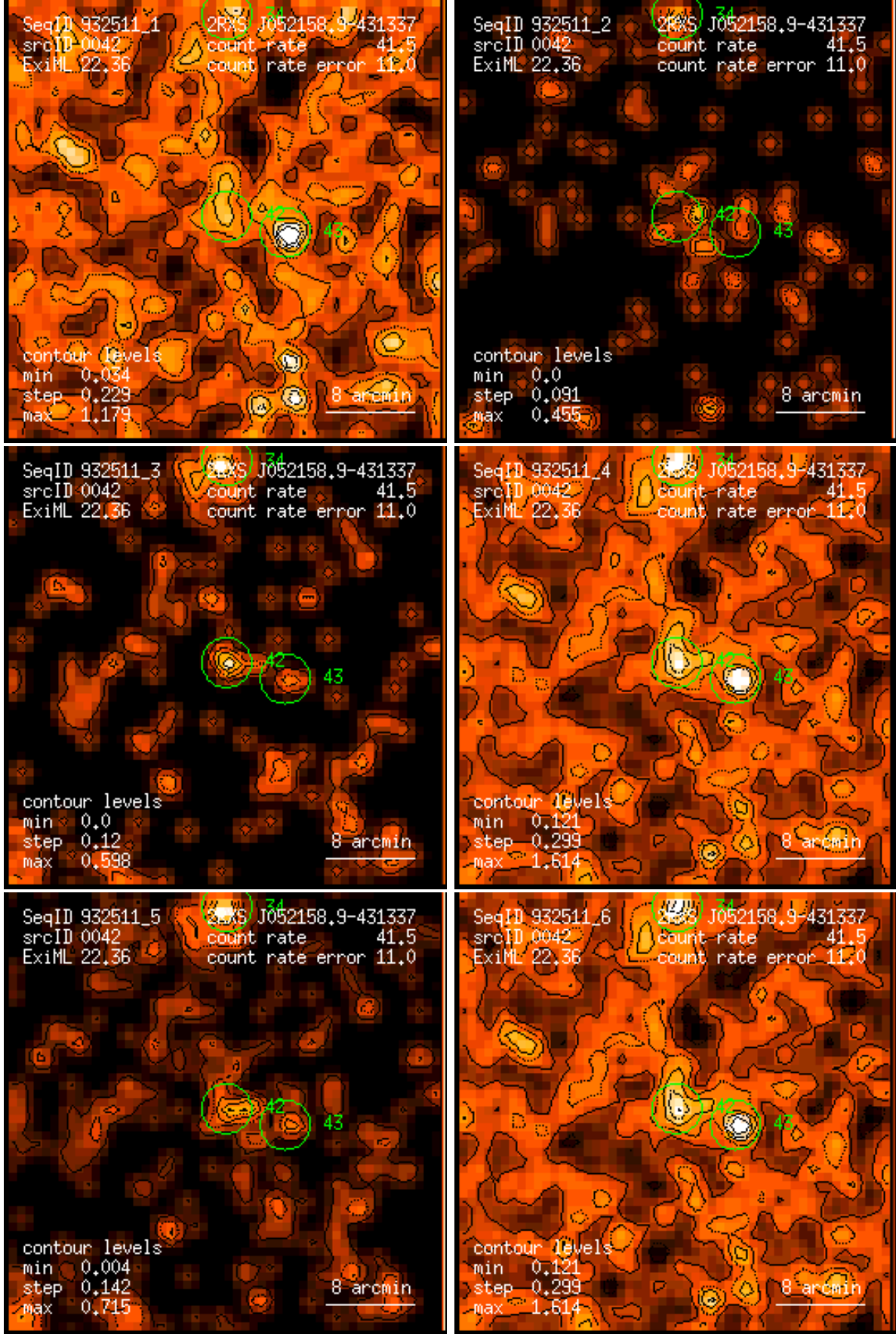
Figure 42: RASS 932511: detection 0042: band rate images, Gaussian filter: (1) PSPC channels 11 – 41, (2) 52 – 90, (3) 91 – 201, (4) 11 – 235, (5) 52 – 201, (6) 11 – 201. Broad band rates in counts/ks. Band rate contour levels in counts/ks/arcmin 2 .
