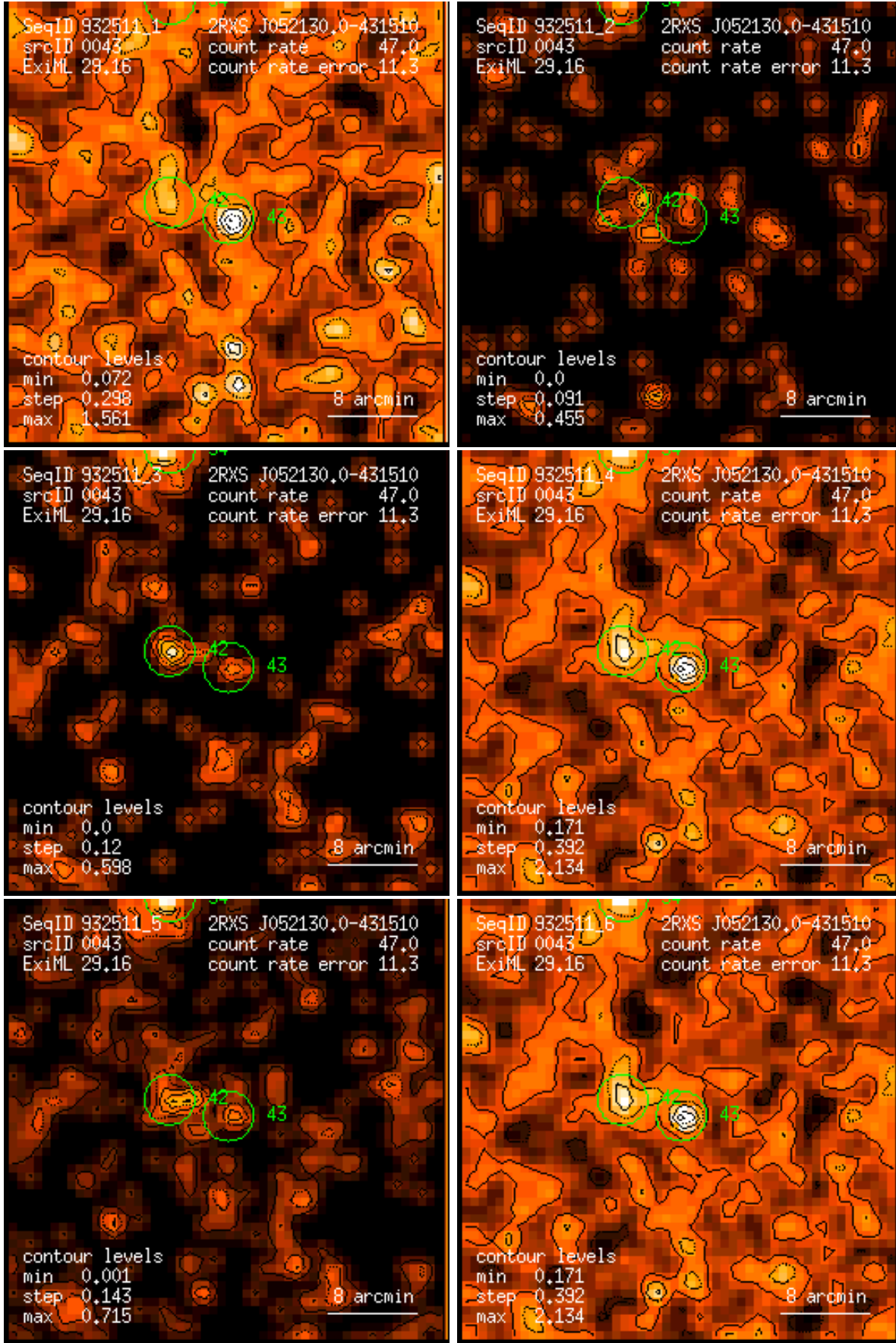
Figure 43: RASS 932511: detection 0043: band rate images, Gaussian filter: (1) PSPC channels 11 – 41, (2) 52 – 90, (3) 91 – 201, (4) 11 – 235, (5) 52 – 201, (6) 11 – 201. Broad band rates in counts/ks. Band rate contour levels in counts/ks/arcmin 2 .
