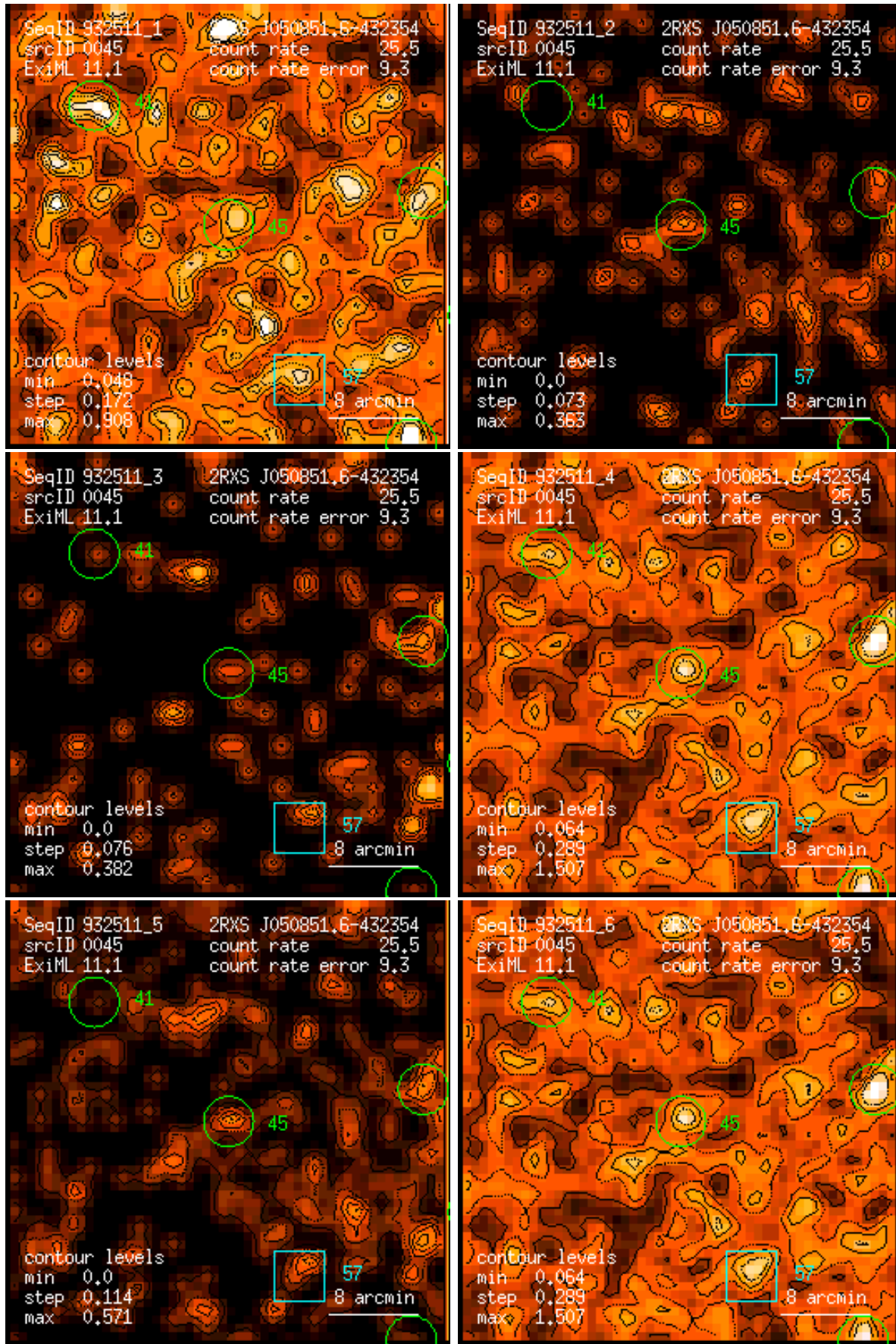
Figure 45: RASS 932511: detection 0045: band rate images, Gaussian filter: (1) PSPC channels 11 – 41, (2) 52 – 90, (3) 91 – 201, (4) 11 – 235, (5) 52 – 201, (6) 11 – 201. Broad band rates in counts/ks. Band rate contour levels in counts/ks/arcmin 2 .
