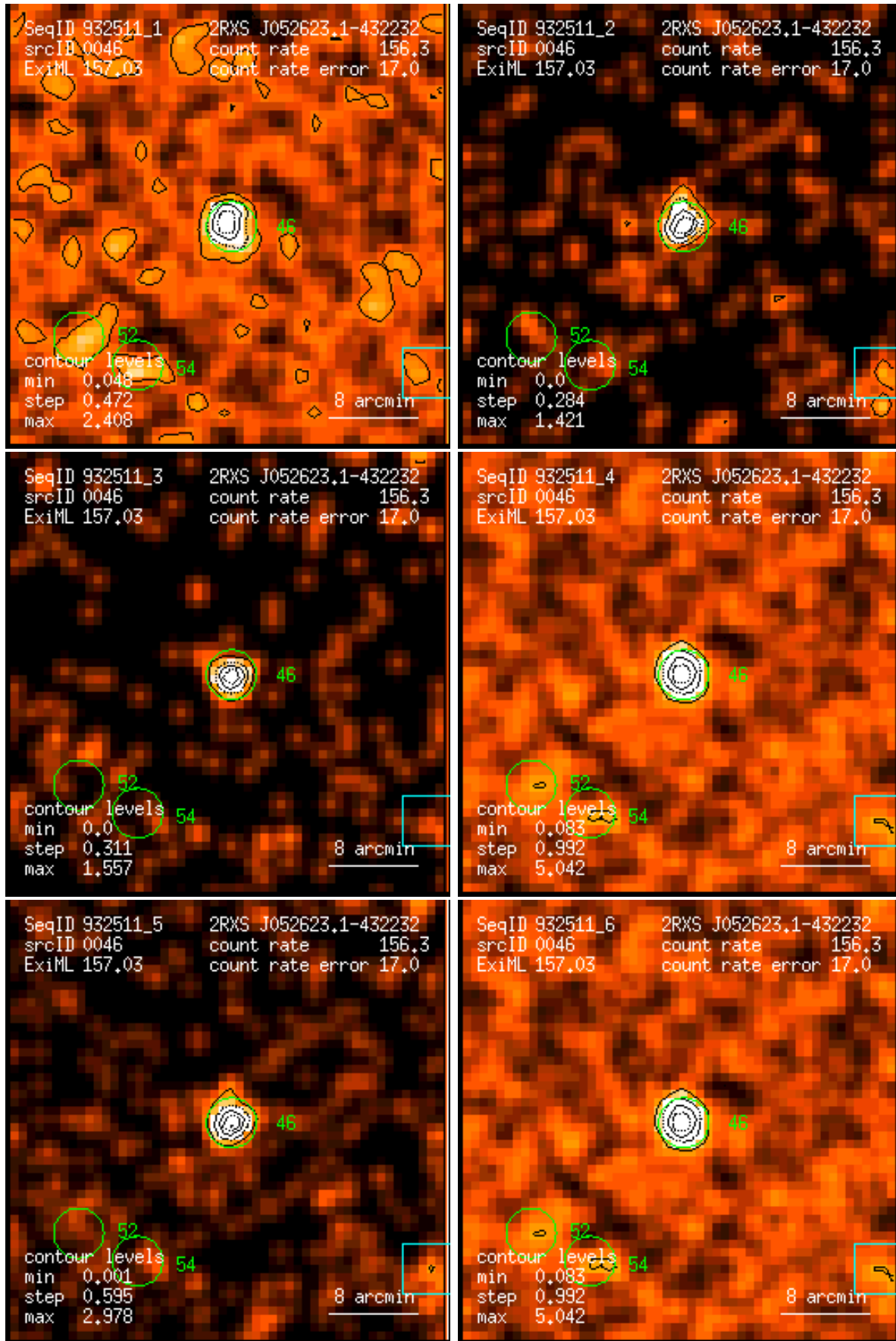
Figure 46: RASS 932511: detection 0046: band rate images, Gaussian filter: (1) PSPC channels 11 – 41, (2) 52 – 90, (3) 91 – 201, (4) 11 – 235, (5) 52 – 201, (6) 11 – 201. Broad band rates in counts/ks. Band rate contour levels in counts/ks/arcmin 2 .
