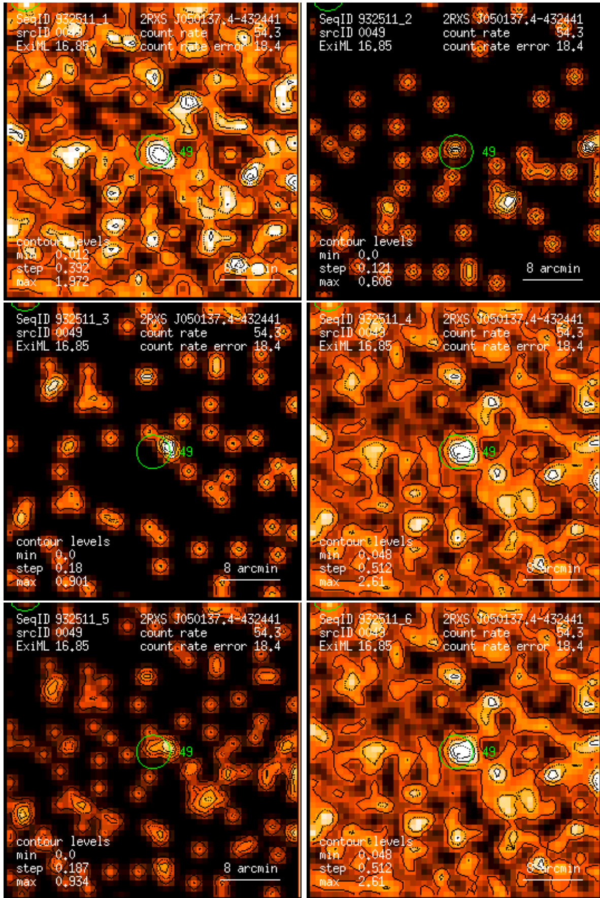
Figure 49: RASS 932511: detection 0049: band rate images, Gaussian filter: (1) PSPC channels 11 – 41, (2) 52 – 90, (3) 91 – 201, (4) 11 – 235, (5) 52 – 201, (6) 11 – 201. Broad band rates in counts/ks. Band rate contour levels in counts/ks/arcmin 2 .
