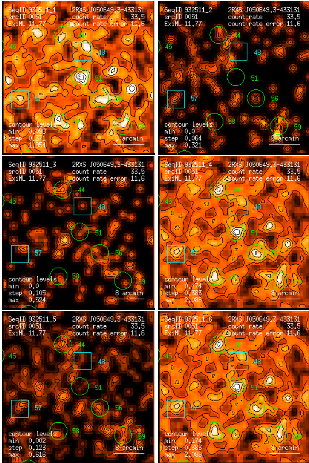
Figure 51: RASS 932511: detection 0051: band rate images, Gaussian filter: (1) PSPC channels 11 – 41, (2) 52 – 90, (3) 91 – 201, (4) 11 – 235, (5) 52 – 201, (6) 11 – 201. Broad band rates in counts/ks. Band rate contour levels in counts/ks/arcmin 2 .
