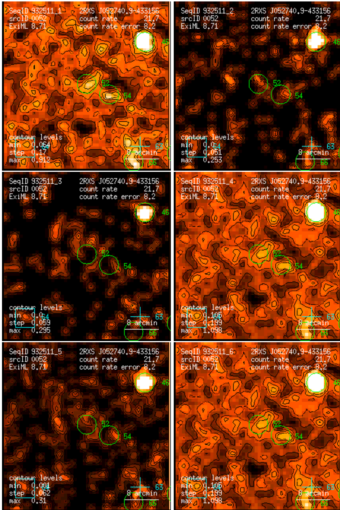
Figure 52: RASS 932511: detection 0052: band rate images, Gaussian filter: (1) PSPC channels 11 – 41, (2) 52 – 90, (3) 91 – 201, (4) 11 – 235, (5) 52 – 201, (6) 11 – 201. Broad band rates in counts/ks. Band rate contour levels in counts/ks/arcmin 2 .
