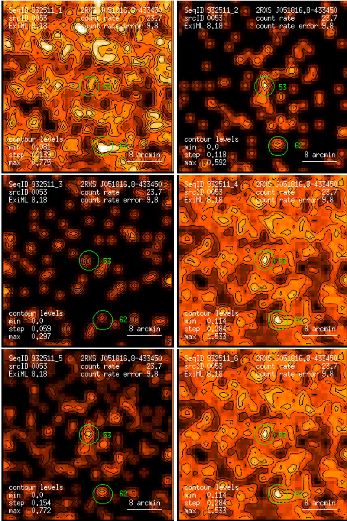
Figure 53: RASS 932511: detection 0053: band rate images, Gaussian filter: (1) PSPC channels 11 – 41, (2) 52 – 90, (3) 91 – 201, (4) 11 – 235, (5) 52 – 201, (6) 11 – 201. Broad band rates in counts/ks. Band rate contour levels in counts/ks/arcmin 2 .
