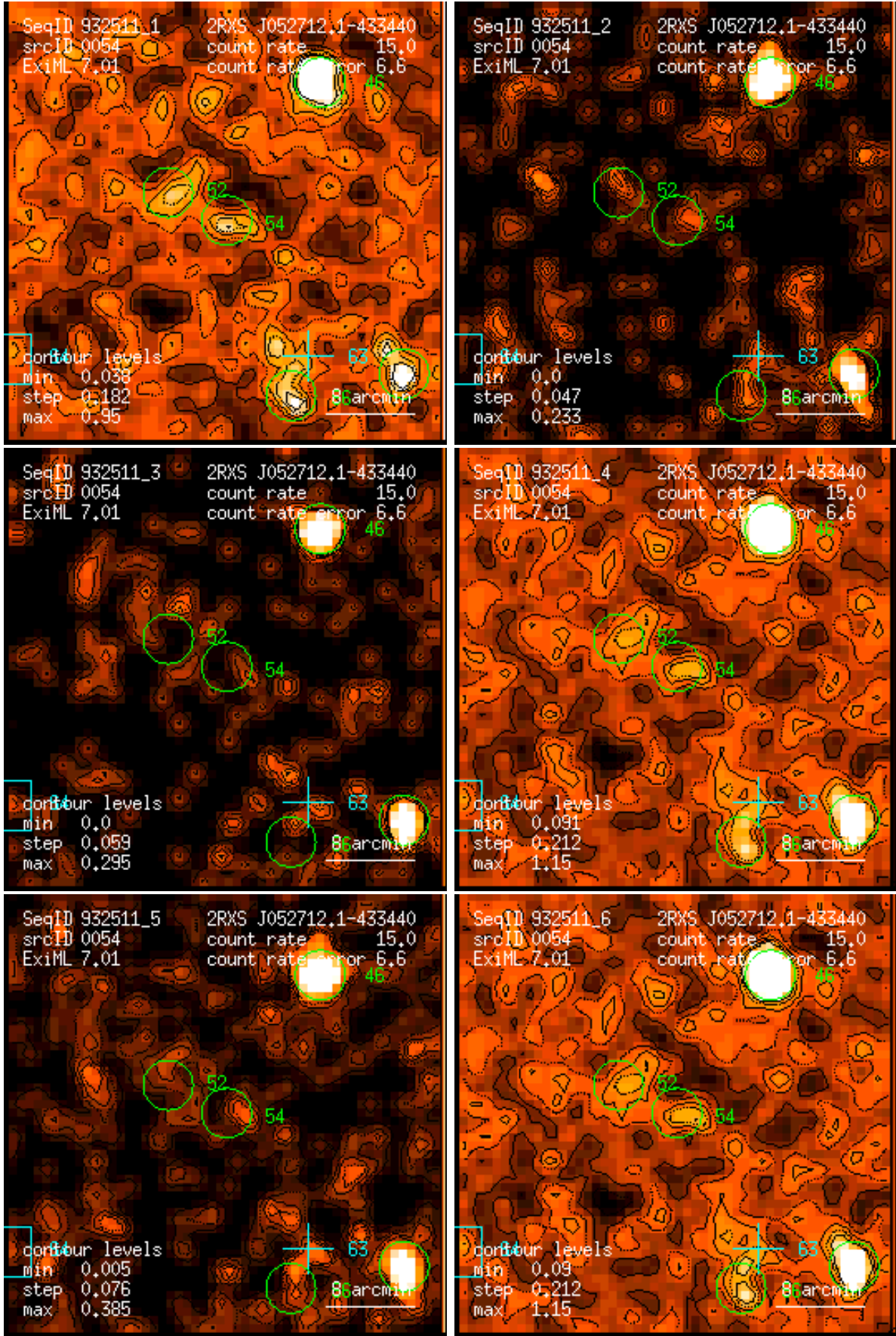
Figure 54: RASS 932511: detection 0054: band rate images, Gaussian filter: (1) PSPC channels 11 – 41, (2) 52 – 90, (3) 91 – 201, (4) 11 – 235, (5) 52 – 201, (6) 11 – 201. Broad band rates in counts/ks. Band rate contour levels in counts/ks/arcmin 2 .
