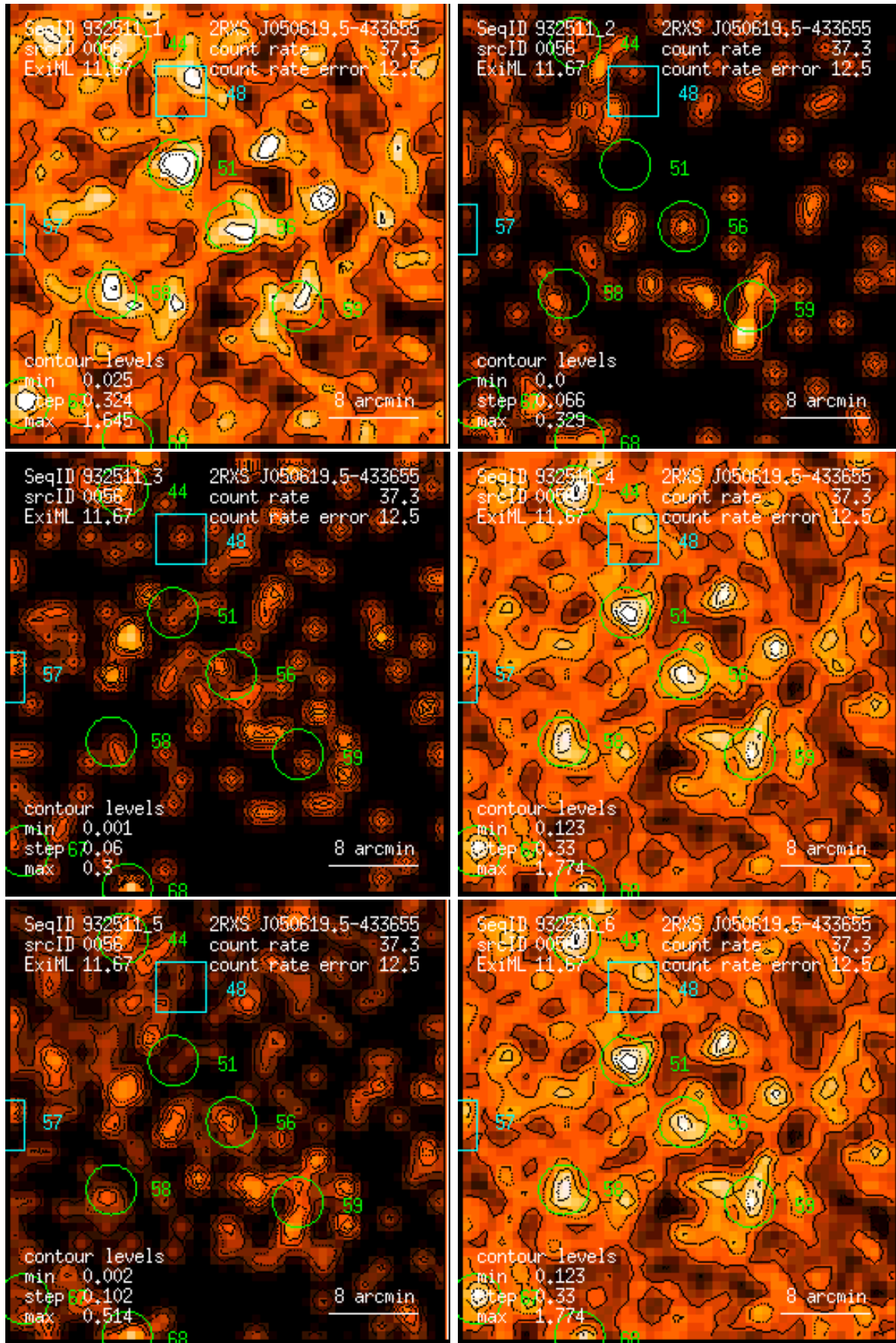
Figure 56: RASS 932511: detection 0056: band rate images, Gaussian filter: (1) PSPC channels 11 – 41, (2) 52 – 90, (3) 91 – 201, (4) 11 – 235, (5) 52 – 201, (6) 11 – 201. Broad band rates in counts/ks. Band rate contour levels in counts/ks/arcmin 2 .
