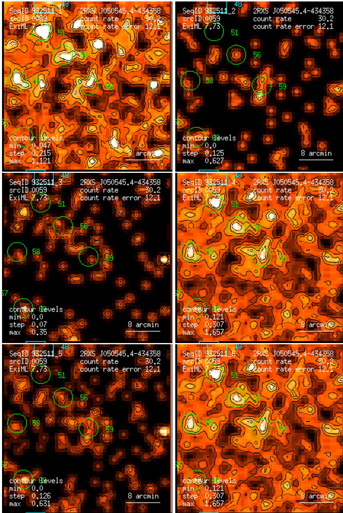
Figure 59: RASS 932511: detection 0059: band rate images, Gaussian filter: (1) PSPC channels 11 – 41, (2) 52 – 90, (3) 91 – 201, (4) 11 – 235, (5) 52 – 201, (6) 11 – 201. Broad band rates in counts/ks. Band rate contour levels in counts/ks/arcmin 2 .
