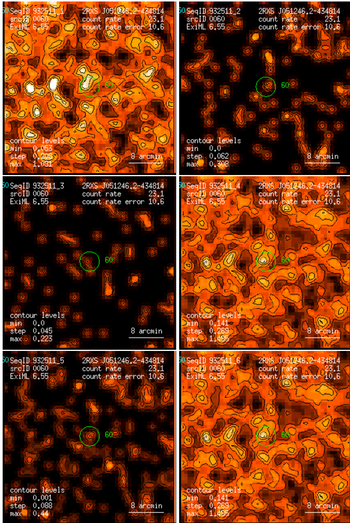
Figure 60: RASS 932511: detection 0060: band rate images, Gaussian filter: (1) PSPC channels 11 – 41, (2) 52 – 90, (3) 91 – 201, (4) 11 – 235, (5) 52 – 201, (6) 11 – 201. Broad band rates in counts/ks. Band rate contour levels in counts/ks/arcmin 2 .
