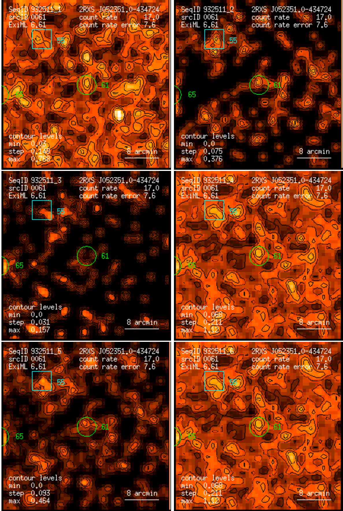
Figure 61: RASS 932511: detection 0061: band rate images, Gaussian filter: (1) PSPC channels 11 – 41, (2) 52 – 90, (3) 91 – 201, (4) 11 – 235, (5) 52 – 201, (6) 11 – 201. Broad band rates in counts/ks. Band rate contour levels in counts/ks/arcmin 2 .
